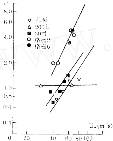
图4 L=190 不同格栅下游湍流速度随来流速度的变化 Fig.4 The turbulence against freestream velocity for 5 kinds of grids at L=190
