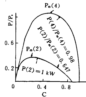
Fig. 7 output power ~ geometric coupling factor (A CO 2 laser)
