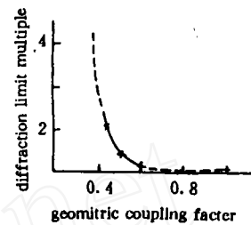
Fig. 3 Geometric coupling factor ~ diffraction limit multiple
