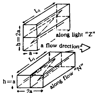
Fig. 5 The light paths in the 3 paths folded cavities
