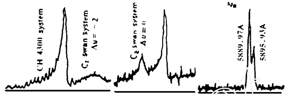
Fig. 8 Visible emission spectra in a wake region of CH 4 /AIR counterflow diffusion flame
