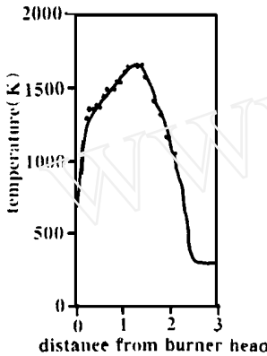
Fig. 3 Temperature profile in a stagnation region of counterflow diffusion flame
