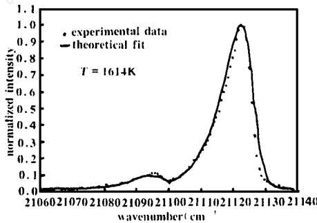
Fig. 4 Comparison between experimental data and theoretical fitting curve
