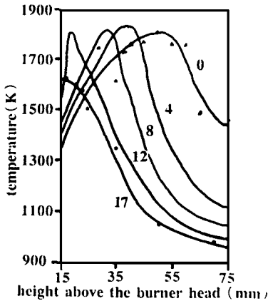
Fig. 5 Temperature distribution at different distance from center line in a wake region of counterflow diffusion flame experimental data: , along center line 0, 17mm far from center line
