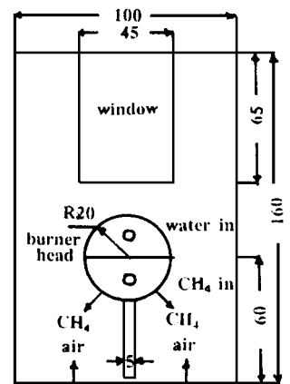
Fig. 2 Diagram of burner
