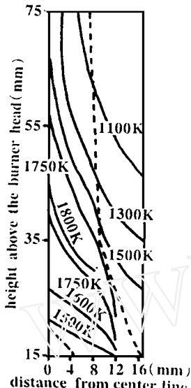
Fig. 7 The 2D temperature distribution in a wake region of counterflow diffusion flame --- flame edges
