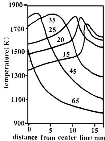
Fig. 6 Temperature distribution at different height in a wake region of counterflow diffusion flame
