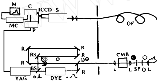
Fig. 1 Schematic illustration of the USED CARS experimental arrangement
