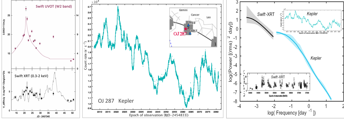
Figure 2: Left panel: Swift XRT X-ray and UVOT UV light curves during the predicted impact outburst epoch for OJ 287 of Nov.-Dec. 2015. The model foreseen the separation of the disk bremsstrahlung (optical and UV flux) from erratic in-jet synchrotron/inverse-Compton beamed variability (X-ray flux). The orphan optical-UV outburst strengthened the evidence for an extra, optical-UV, out of the jet, emission (adapted from [14]). Central panel: the 1-minute sampling optical light curve from Apr. 27 to Jul. 13, 2015 of OJ 287 obtained by the Kepler space telescope (K2 mission, Campaign #5). Right panel: temporal variability power density spectrum of OJ 287 constructed with Kepler and Swift data (adapted from [2]).
