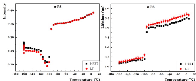
Fig. 4. Results of the hexane scan shown as dependence of o -positronium lifetime and intensity over temperature. In the left part, data from LT and J-PET software above -100^{\circ}\text{C} are superimposed.
