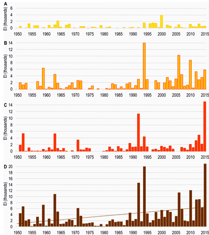
Figure 14. Long-term courses of the monthly and seasonal means of the extremity index (°C·km 2 ) (1951–2015): (A) June, (B) July, (C) August, (D) summer season (dotted line—linear trend).
