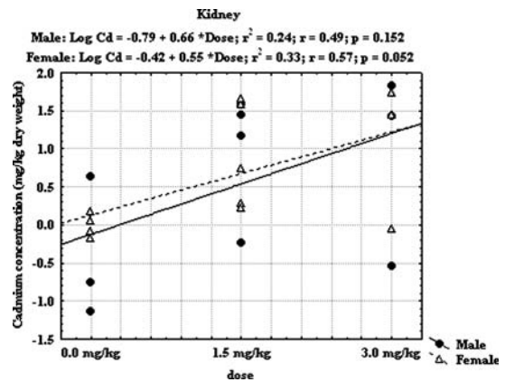
Figure 4. The relationship between the Cd dose (mg/kg body mass) and concentrations of cadmium (mg/kg dry weight) in the kidney of male and female bank voles. The regression lines for male (solid line) and female (dashed line) are shown.
