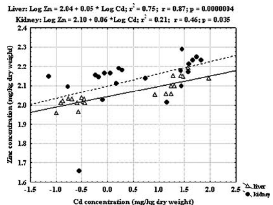
Figure 5. The relationship between the Cd and Zn concentrations (mg/kg dry weight) in the liver and kidney's of bank voles. The regression lines for the liver (solid line) and kidney (dashed line) are shown.
