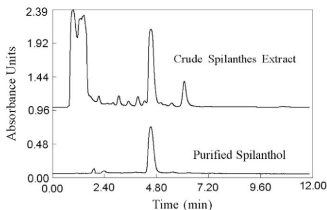
Fig. 3. HPLA chromatograms showing alkylamide content of raw (100% ethanol) Spilanthes acmella extract and a sample of spilanthol purified from the crude extract. Spilanthol is the primary alkylamide component of the raw extract.
