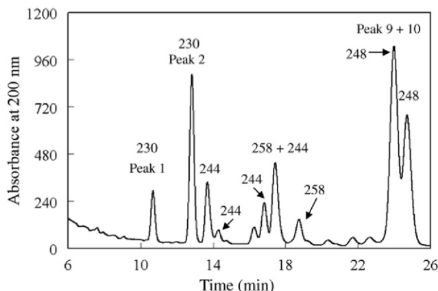
Fig. 2. HPLC chromatogram showing the relative abundance of 11 different alkylamides from a 100% ethanol extract from Echinacea purpurea . The molecular weight of each of the components was determined by isolating the fractions containing that peak and subjecting them to ESI-MS analysis. The molecular weights of the protonated molecular ion that corresponds to each peak is indicated on the chromatogram. It should be noted that these molecular weights are one larger than the weights shown in Fig. 1 because of the additional mass of the proton.
