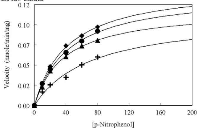
Fig. 4. Michaelis-Menton plots showing the inhibition of cytochrome P450 2E1 -dependent oxidation of p -nitrophenol by (+) hydrastine, (●) canadine, and (▲) berberine, in pooled human liver microsomes. Activities are compared to the control reaction (◆) in which no inhibitor was present.
