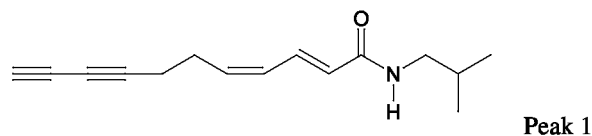
Undeca-2E,4Z-diene-8,10-diyonic acid isobutylamide MW = 229.32 g/mole
