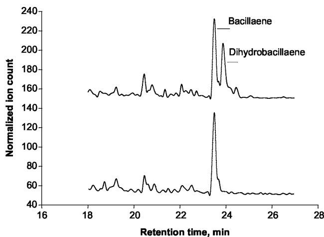
Fig. 4. Partial LC-MS chromatograms of ATCC 39374 extracts. Top trace, LC-MS of untreated ATCC 39374 methanolic extracts; Bottom trace, LC-MS of the same extract treated with PksS, crude reductase, and NADH. Traces are offset for clarity.
