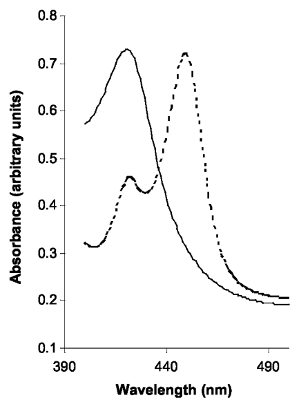
Fig. 3. Visible electronic absorption spectra of PksS. The ferric (solid) and reduced-CO complex (dashed) of the PksS gene product.
