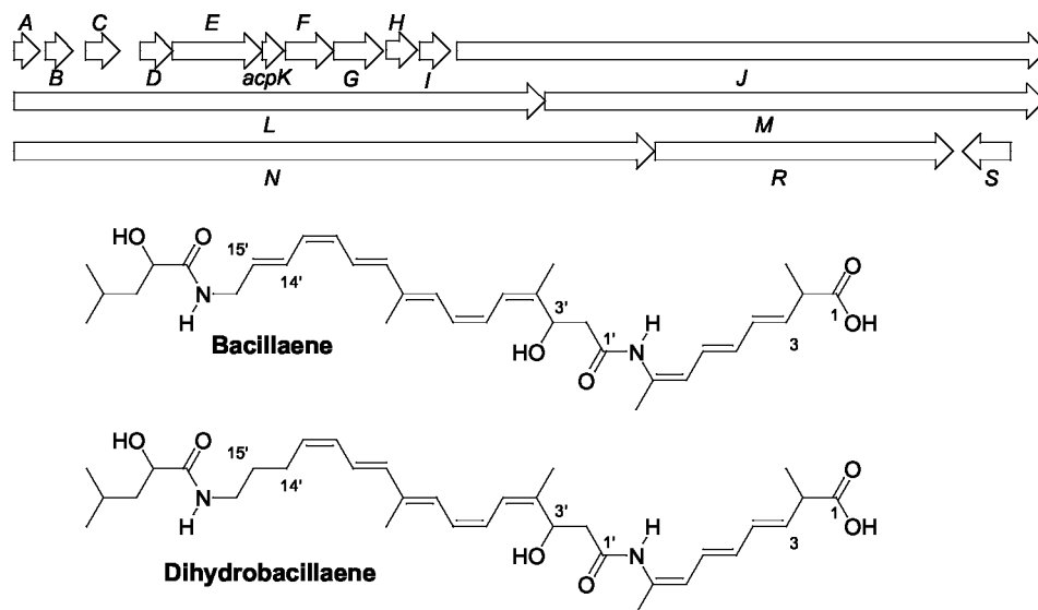
Fig. 1. The pksX gene cluster of Bacillus subtilis strain 168, and the structures of bacillaene and dihydrobacillaene. Functional assignments of pksX genes are given in the text.
