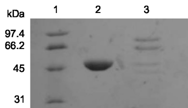
Fig. 2. SDS-PAGE of purified PksS protein. Lane 1: molecular weight markers. Lane 2: PksS obtained after Ni-NTA chromatography. Lane 3: post-induction crude extract of M15[pREP4] which had overexpressed pQE60-pksS.
