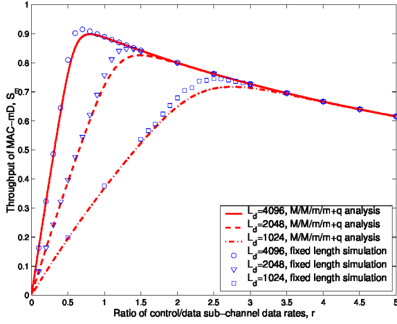
Fig. 11. Simulation and analytical results of the throughput of the MAC-mD schemes for m = 8 , q = 8 , different values of L_d , and for the fixed-total-bandwidth scenario
