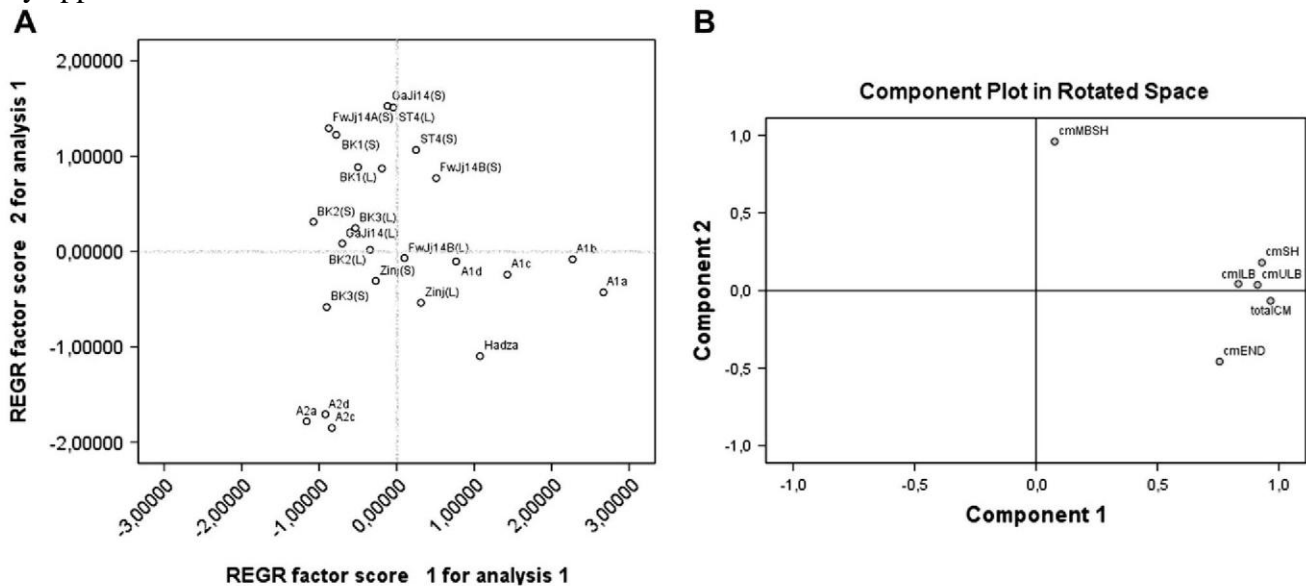
Figure 22. Principal components analysis of the Plio-Pleistocene archaeological assemblages and the experimental samples shown in Table 14. A1, primary access experiments; A2, secondary access experiments (Domínguez-Rodrigo, 1997b). Notice the separate cluster formed by the experiments replicating passive scavenging of defleshed carcasses (A2). The primary access experiments show a wider scatter given that two butchering processes are included: thorough defleshing of all flesh scraps (A1a,b,c) and regular butchering neglecting small flesh scraps (A1d and Hadza) (Domínguez-Rodrigo, 1997a, b; Lupo and O'Connell, 2002). The determinant value is 0.003; the KMO measure of sampling adequacy is 0.74; and the eigenvalues of both factors explain 85% of the sample variance. Key: cmTotal, cut-marked percentage of long bone specimens; cmSH, cut-marked shafts; cmEND, cut-marked epiphyseal fragments; cmULB, cut-marked upper limb bones; cmILB, cut-marked intermediate limb bones; cmMBSH, cut-marked meat-bearing long bone shafts. For the regression factor score: (S), small carcasses (Bunn's sizes 1 and 2); (L), large carcasses (Bunn's size 3).
