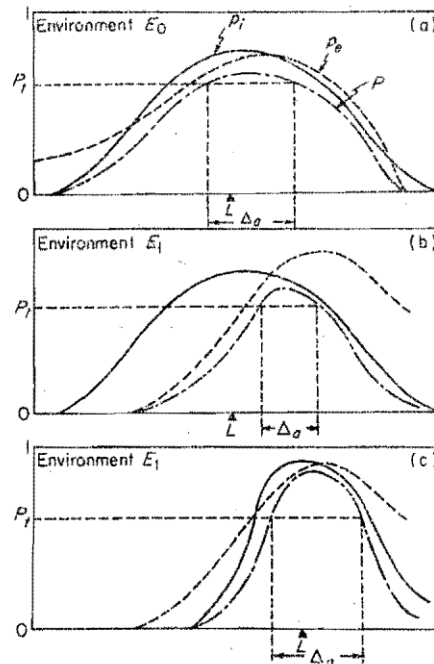
FIG. 5. Mechanism of change in the legisign under changing environmental conditions. In each diagram, the solid curve represents the probability ( p_i ) of a sinsign expressing the correct interpretant if it is received with no equivocation, the broken curve the probability ( p_e ) of error-free transmission and the semi-broken curve the probability ( P ) of a sinsign expressing the correct interpretant under the particular environmental conditions. "L" indicates the position of the legisign in each case.
