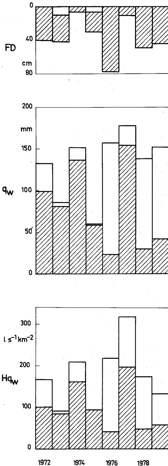
Fig. 4. Spring runoff ( q_w ) and spring maximum runoff ( Hq_w ) from sub-drains (hatched) and surface (unhatched) in the Hovi basin after sub-drainage. FD indicates the depth of soil frost during the spring maximum runoff.
