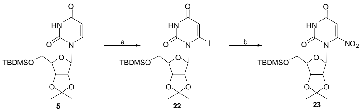
Scheme 12. Attempted synthesis for the formation of 6-nitro from fully protected 6-iodo derivative. Reactions conditions: (a) LDA, THF, iodine, -78\text{ }^{\circ}\text{C} (b) DMF, copper powder, tetrabutylammonium nitrite, N,N' -dimethylethylenediamine, 100\text{ }^{\circ}\text{C} .
