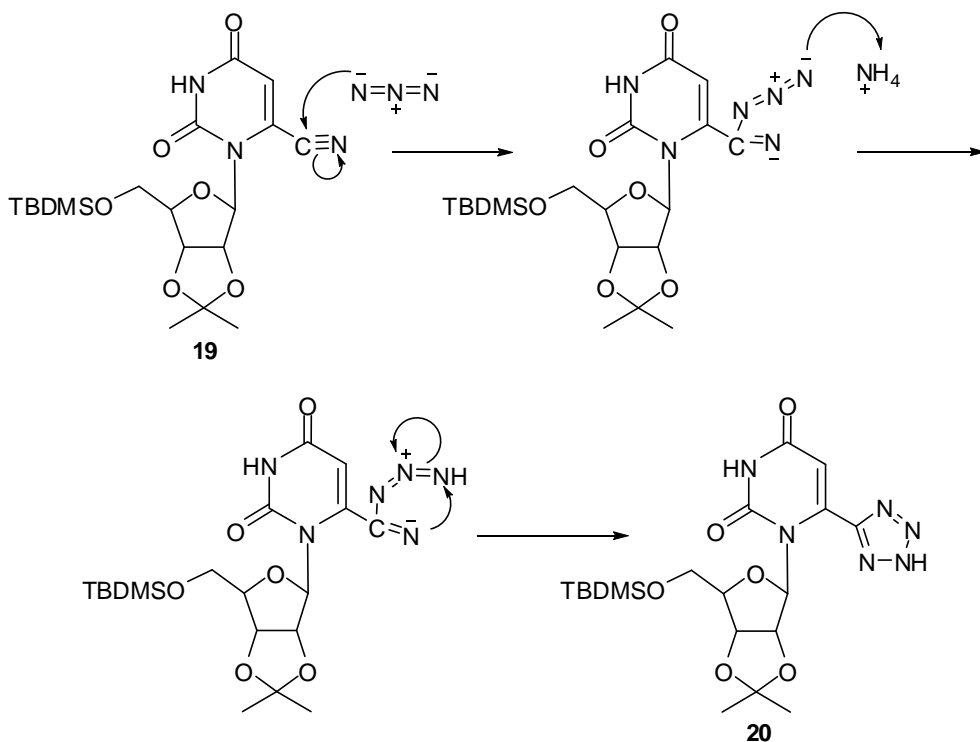
Scheme 10. Reaction mechanism for the formation of 6-tetrazole from the fully protected 6-cyano uridine derivative.
