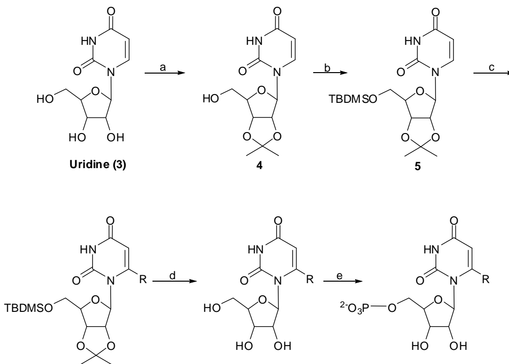
Scheme 3. General scheme for synthesis of C6 derivatives of UMP. Reaction conditions: a) acetone, \text{H}_2\text{SO}_4 b) \text{CH}_2\text{Cl}_2 , imidazole, TBDMSCl, 0\text{ }^\circ\text{C}\rightarrow\text{RT} c) Specific to derivative d) 50% trifluoroacetic acid in \text{H}_2\text{O} , 0\text{ }^\circ\text{C}\rightarrow\text{RT} e) \text{H}_2\text{O} , \text{POCl}_3 , acetonitrile, pyridine, 0\text{ }^\circ\text{C} , \text{NH}_4\text{OH} .
