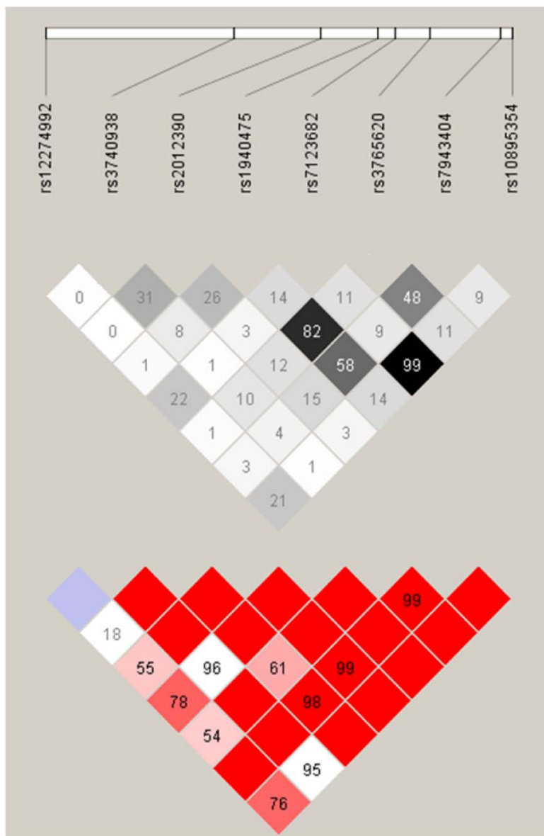
Figure 9. The LD block structure of the MMP8 gene in the Finnish controls of the Finnish discovery knee OA sample. Above the r^2 measure of LD, below the D' measure of LD. The pair-wise LD is shown as different shadings of grey ( r^2 ) and red ( D' ) (Barrett et al. 2005).
