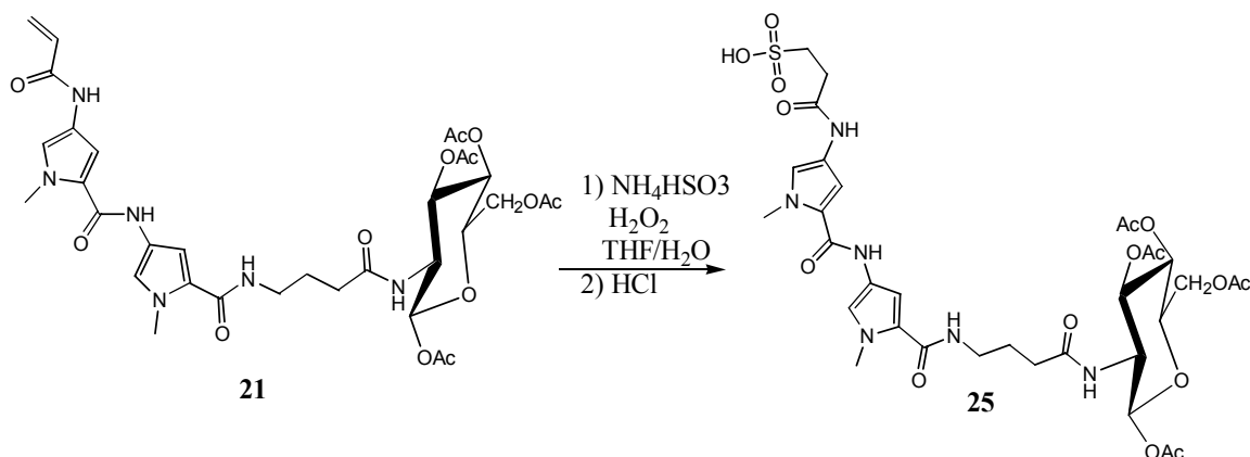
Scheme 3.19
