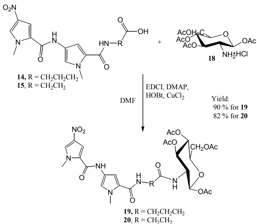
Scheme 3.16
