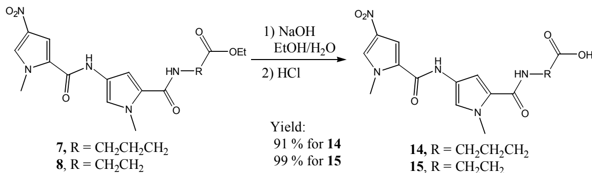
Scheme 3.14
