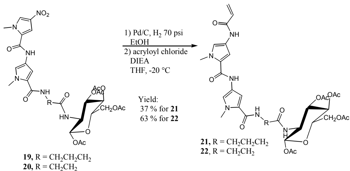
Scheme 3.17
