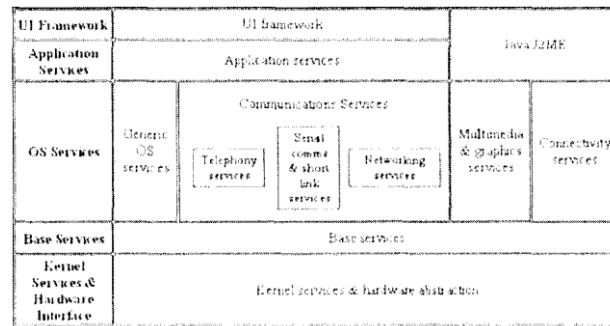
Fig. 8. Symbian OS architecture.
