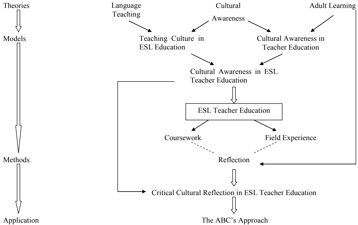
Figure 1. Theoretical Framework
