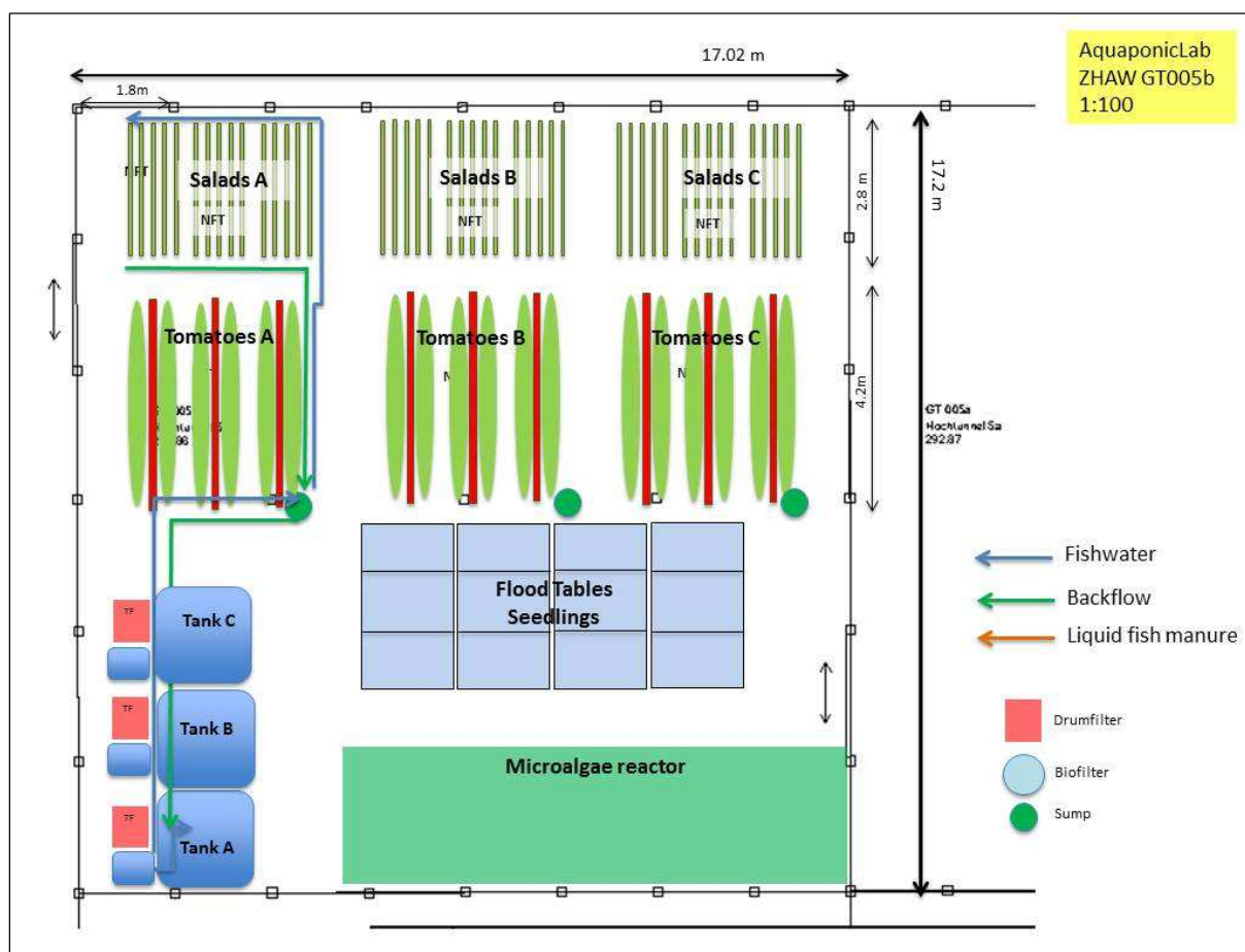
Figure 2: Floor plan of the Aquaponic research and training facility.
