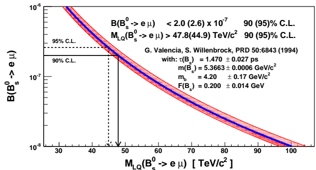
FIG. 3: Leptoquark mass limit corresponding to the 90 (95) % C.L. on \mathcal{B}(B_s^0 \rightarrow e^+\mu^-) . The error band is obtained by varying the values entering the theoretical calculation within their uncertainties. The uncertainties stemming from approximating \alpha_s are not included.
