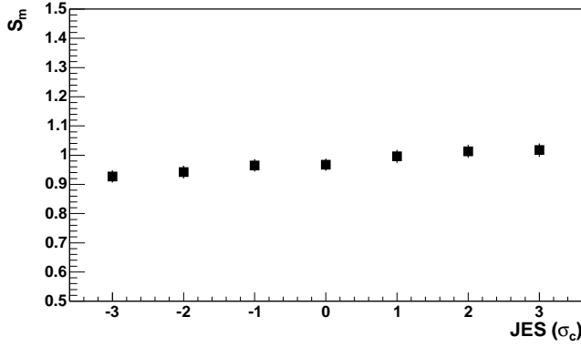
FIG. 18: Distribution of parameter S_m (Eq. 41) as a function of JES.
