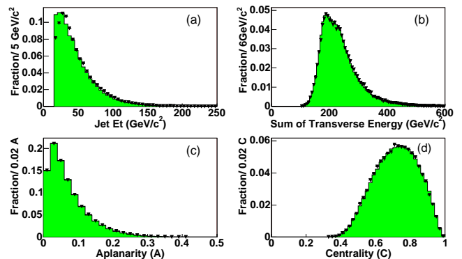
FIG. 7: Background validation in control region CR1 for single tagged events from the multi-jet data (dots) and from the background model (solid histogram). The distributions are normalized to the same area.
