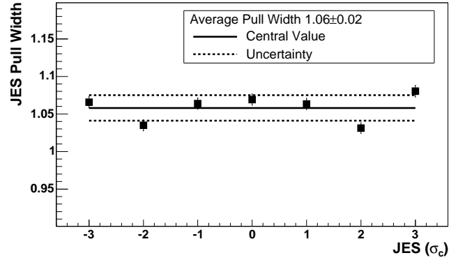
FIG. 24: Pull widths versus JES_{true} in the case of the reconstruction of JES in samples with M_{top} = 170 \text{ GeV}/c^2 . The continuous line represents the average pull width and the dashed lines show the uncertainty on it.
