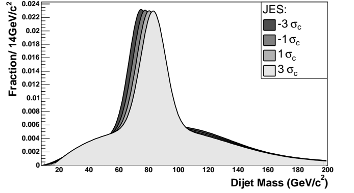
FIG. 14: The function fitting the dijet mass templates for t\bar{t} events with M_{top} = 170 \text{ GeV}/c^2 and various values of JES in the case of events with one tagged jet. A similar parameterization is obtained for events with at least two tagged jets.
