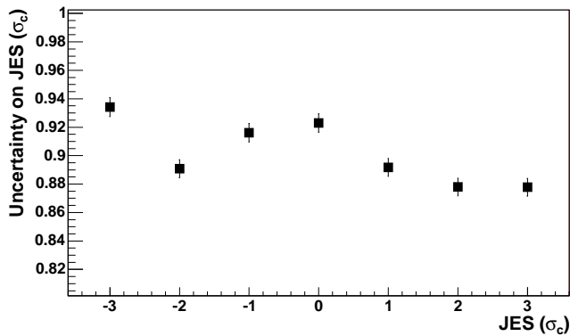
FIG. 26: Expected uncertainty on JES, \delta JES_{out} , versus JES_{true} , for samples with M_{top} = 170 \text{ GeV}/c^2 .
