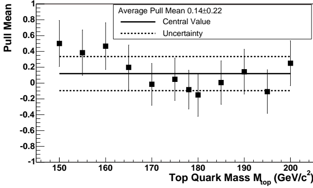
FIG. 21: Pull means versus M_{top} in the case of the reconstruction of top quark mass in samples with JES_{true} = 0 \sigma_c . The continuous line represents the average pull mean and the dashed lines show the uncertainty on it.
