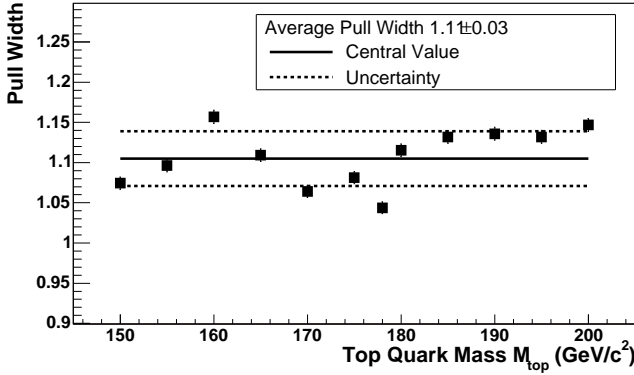
FIG. 22: Pull widths versus M_{top} in the case of the reconstruction of top quark mass in samples with JES_{true} = 0 \sigma_c . The continuous line represents the average pull width and the dashed lines show the uncertainty on it.
