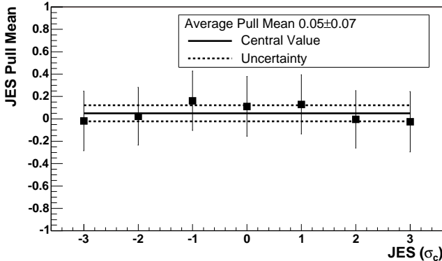
FIG. 23: Pull means versus JES_{true} in the case of the reconstruction of JES in samples with M_{top} = 170 \text{ GeV}/c^2 . The continuous line represents the average pull mean and the dashed lines show the uncertainty on it.
