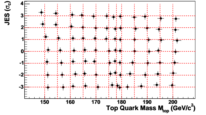
FIG. 16: JES versus Top Quark Mass plane. The points represent the reconstructed JES, JES_{out} , and top quark mass M_t and have attached their corresponding statistical uncertainties, \delta JES_{out} and \delta M_t . The vertical dashed lines correspond to the true values of the mass, while the horizontal lines correspond to the true values of JES. For a perfect reconstruction the points should sit right at the intersection of the dashed lines.
