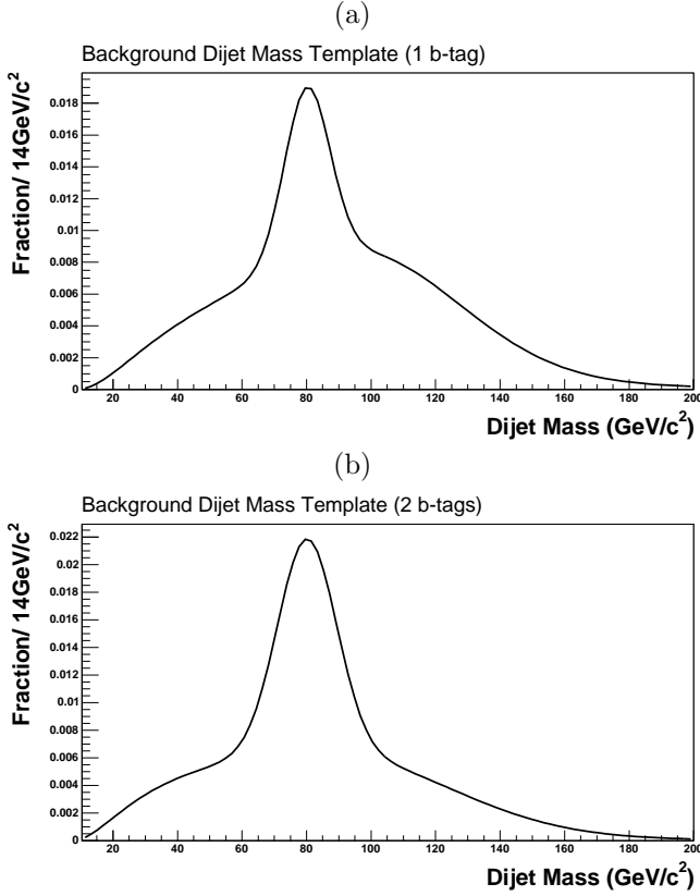
FIG. 15: Dijet mass templates for (a) single tagged background events and for (b) double tagged background events.
