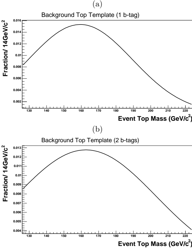
FIG. 13: Top templates for (a) single tagged background events and for (b) double tagged background events.
