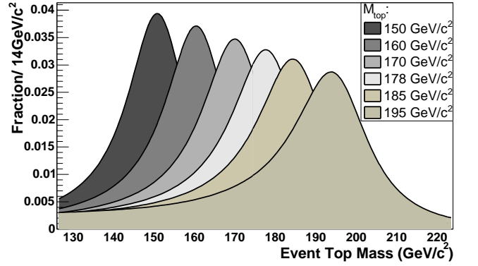
FIG. 12: The function fitting the top templates for t\bar{t} events at nominal JES and for various hypotheses of the top quark mass in the case of events with one tagged jet. A similar parameterization is obtained for events with at least two tagged jets.
