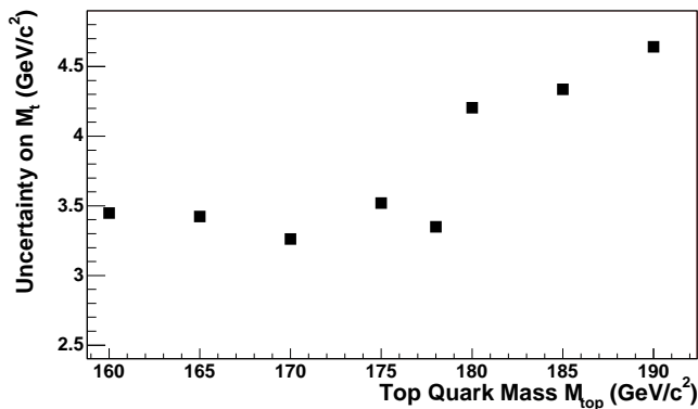
FIG. 25: Expected uncertainty on top quark mass, \delta M_t^{corr} , versus M_{top} , for samples with JES_{true} = 0 \sigma_c . This uncertainty includes the uncertainty due to statistical effects and the systematic uncertainty due to jet energy scale.
