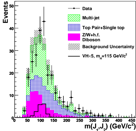
FIG. 2: Dijet invariant mass distribution for double-tagged events in signal region.
