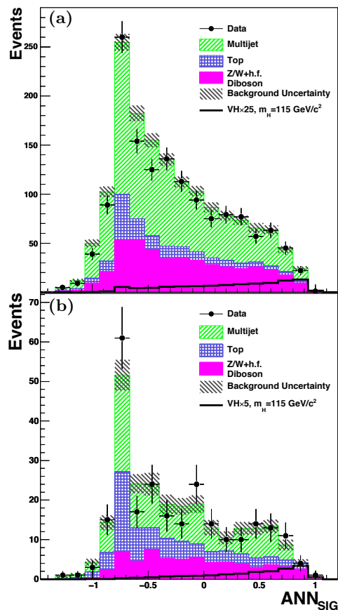
FIG. 3: The distribution of ANN sig for (a) single- and (b) double-tagged events.
