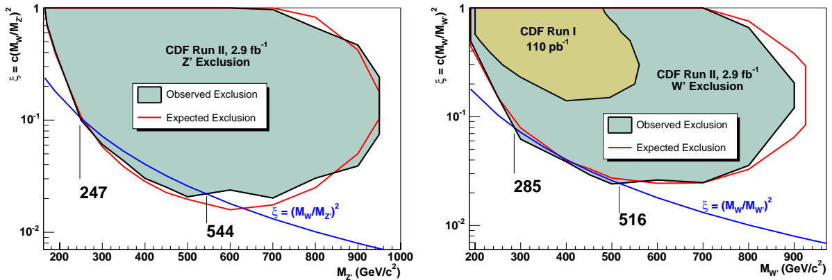
FIG. 4: Z' (left) and W' (right) exclusion regions as a function of mass and \xi . The \xi = (M_W/M_Z)^2 (i.e., C = 1 ) lines indicate PYTHIA defaults and are commonly used for mass exclusion regions. The vertical lines mark the results as shown in Table II. Also shown in the W' plot is the CDF Run I result.
