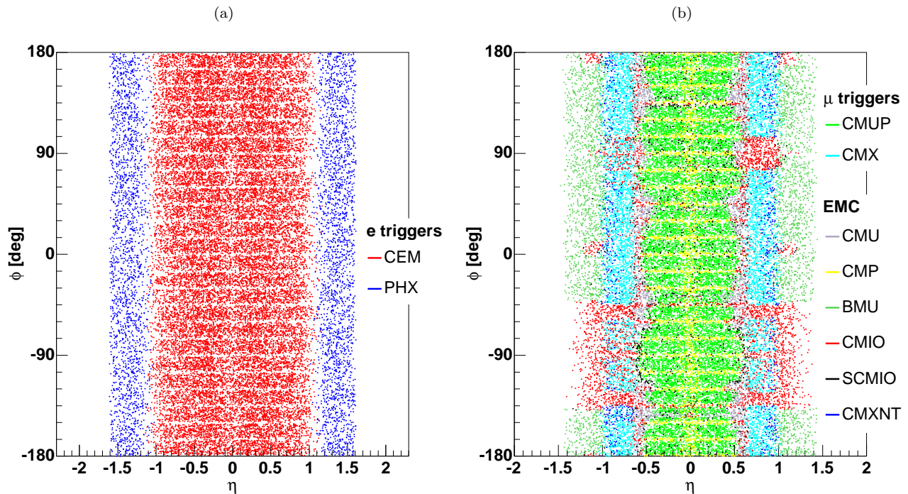
FIG. 4: Distributions in (\phi - \eta) space of the electron (a) and muon (b) selection categories, showing the coverage of the detector that each lepton category provides. The muon categories are more complicated due to the geometrical limitations of the several different muon detectors of CDF.
