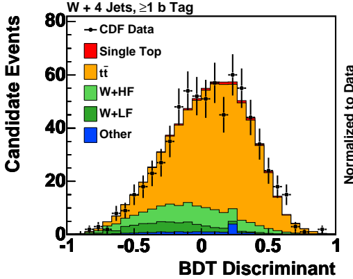
FIG. 32: The BDT output for four-jet events containing one or more b tags. The dominant source of background is t\bar{t} events. The data are indicated with points and the stacked histograms show the prediction, scaled to the total data rate, with the stacking order following that of the legend.
