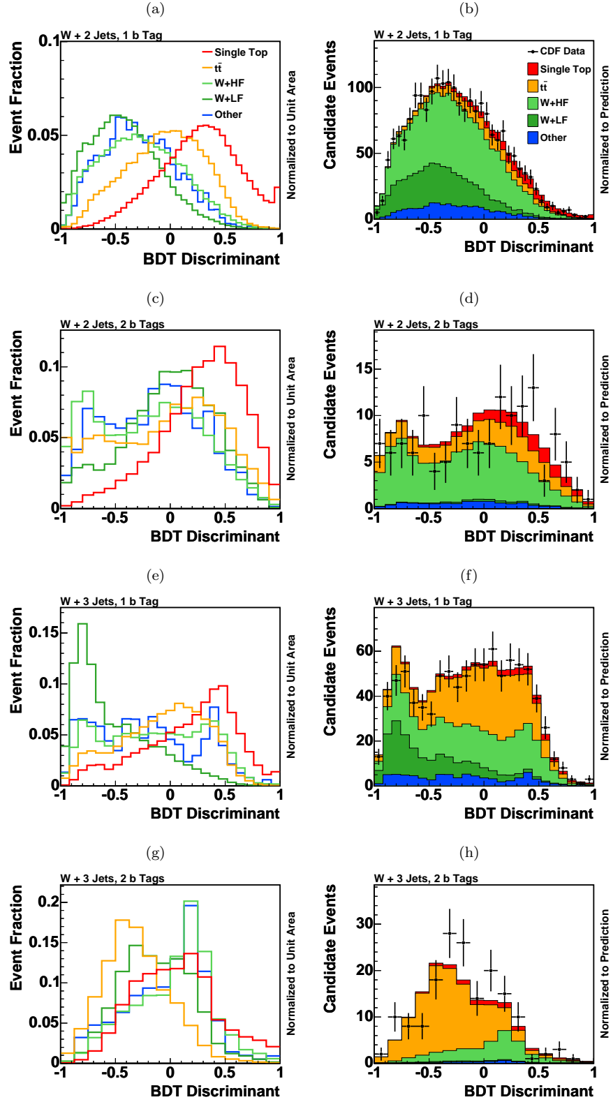
FIG. 30: Templates of predictions for the signal and background processes, each scaled to unit area (left) and comparisons of the data with the sum of the predictions (right) of the boosted decision tree output for each data sample. Single top quark events are predominantly found on the right-hand sides of the histograms while background events are mostly found on the left-hand sides. The data are indicated by points with error bars, and the predictions are shown stacked, with the stacking order following that of the legend.
