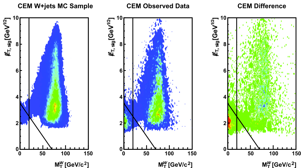
FIG. 5: Plots of \cancel{E}_{T,\text{sig}} vs. M_T^W for W +jets Monte Carlo, the selected data in the \ell + \cancel{E}_T + 2 jets sample, and the two distributions subtracted for all CEM candidates. The black lines indicate the requirements which are applied. Events with lower \cancel{E}_{T,\text{sig}} or M_T^W are not selected.
