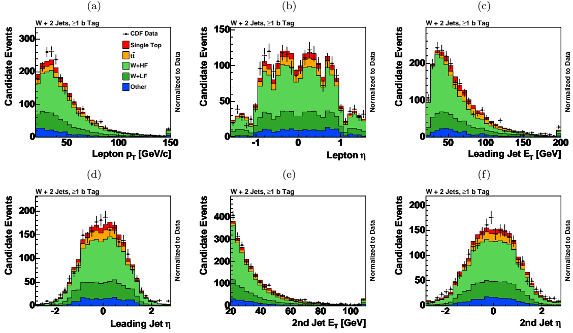
FIG. 16: Validation plots comparing data and Monte Carlo for basic kinematic quantities for events passing the event selection requirements with two jets and at least one b tag. The data are indicated with points, and the shaded histograms show the signal and background predictions which are stacked to form the total prediction. The stacking order follows that of the legend.
