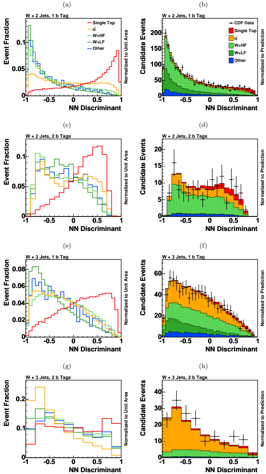
FIG. 27: Templates of predictions for the signal and background processes, each scaled to unit area (left) and comparisons of the data with the sum of the predictions (right) of the neural network output for each signal region. Single top quark events are predominantly found on the right-hand sides of the histograms while background events are mostly found on the left-hand sides. The data are indicated by points with error bars, and the predictions are shown stacked, with the stacking order following that of the legend.
