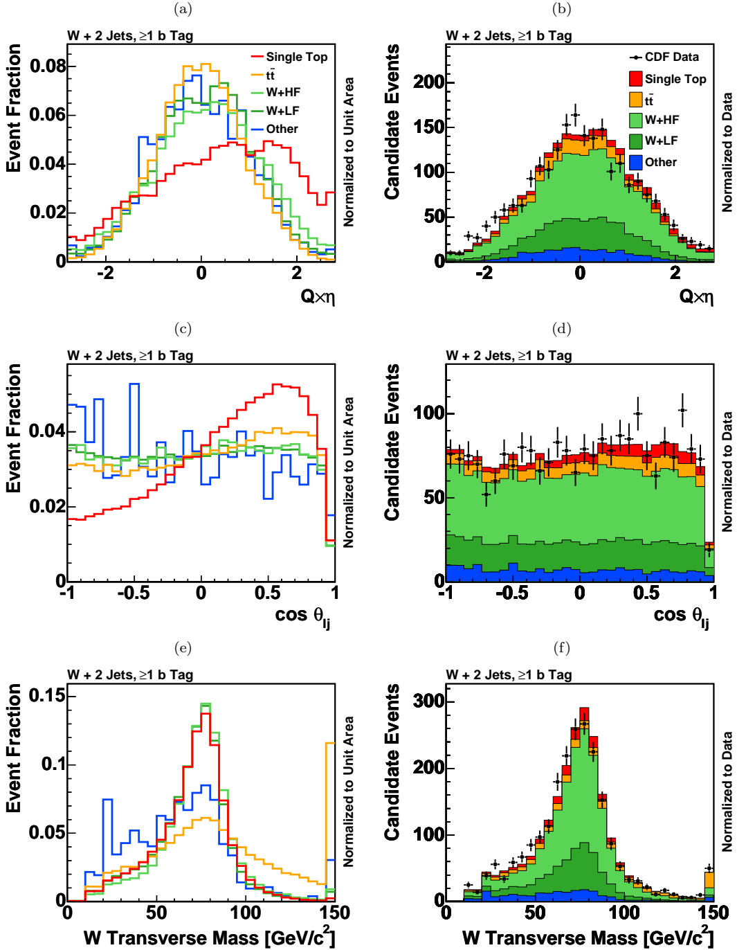
FIG. 20: Monte Carlo templates (left) and validation plots (right) comparing data and Monte Carlo for variables with good discriminating power for events passing our selection requirements with two identified jets and at least one b tag. The data are indicated with points, and the shaded histograms show the signal and background predictions which are stacked to form the total prediction. The stacking order follows that of the legend. Overflows are collected in the highest bin of each histogram.
