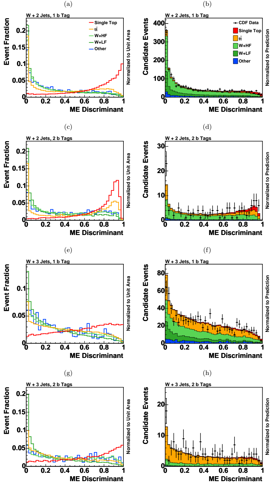
FIG. 24: Templates of predictions for the signal and background processes, each scaled to unit area (left) and comparisons of the data with the sum of the predictions (right) of the ME discriminant EPD for each selected data sample. Single top quark events are predominantly found on the right-hand sides of the histograms while background events are mostly found on the left-hand sides. The data are indicated by points with error bars, and the predictions are shown stacked, with the stacking order following that of the legend.
