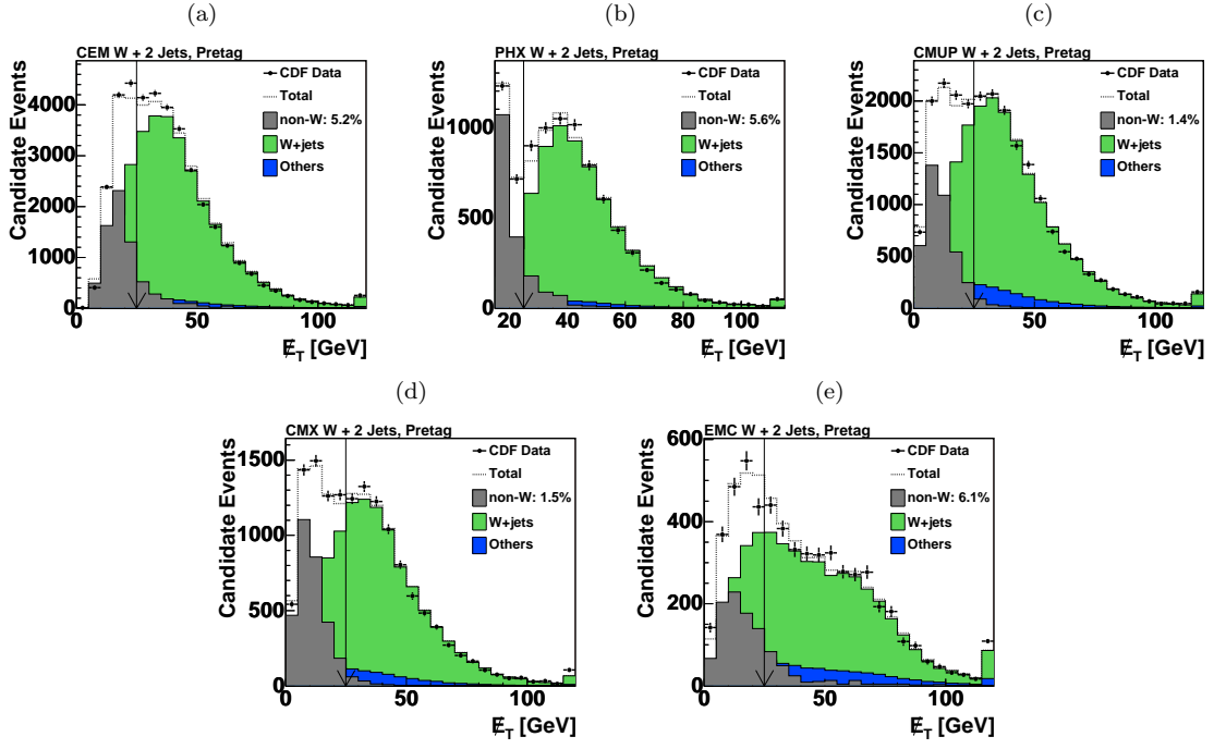
FIG. 12: Fits to E_T distributions in the pretag samples for the five different lepton categories (CEM, PHX, CMUP, CMX, EMC) in W+2 jet events. The fractions of non- W events are estimated from the portions of the templates above the E_T thresholds shown by the arrows. Overflows are collected in the highest bin of each histogram. The data are indicated with points with error bars, and the shaded histograms show the best-fit predictions. The non- W templates are not shown stacked, but the W +jets and “Others” templates are stacked. The unshaded histogram is the sum of the fitted shapes.
