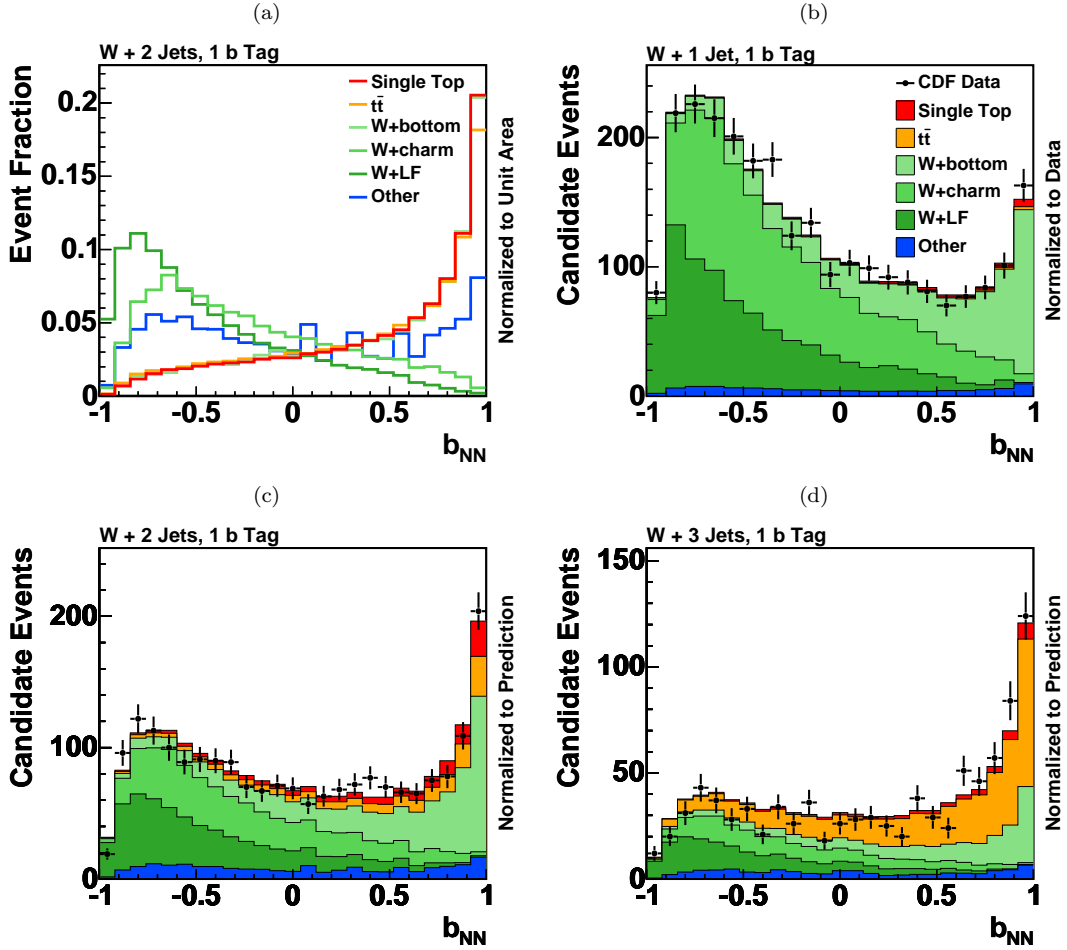
FIG. 14: Templates (a) of the jet flavor separator b_{\text{NN}} for W +light, W +charm (adding the Wc\bar{c} and Wcj contributions because of their similar shapes), and W +bottom events. The template labeled “Other” represents the diboson and Z/\gamma^* +jets contributions. The strong discrimination b_{\text{NN}} provides to separate jet flavors makes it a powerful variable in multivariate analyses. Panel (b) shows the outcome of the fit to the W +1 jet data sample allowing the b , c , and light-flavor components to float as described in Section V. Panels (c) and (d) compare the data and the corresponding predictions in the W +2 jet and W +3 jet samples. In panels (b) through (d), the data are indicated with points with error bars, and the model predictions are shown with shaded histograms, stacked in the same order as the legend.
