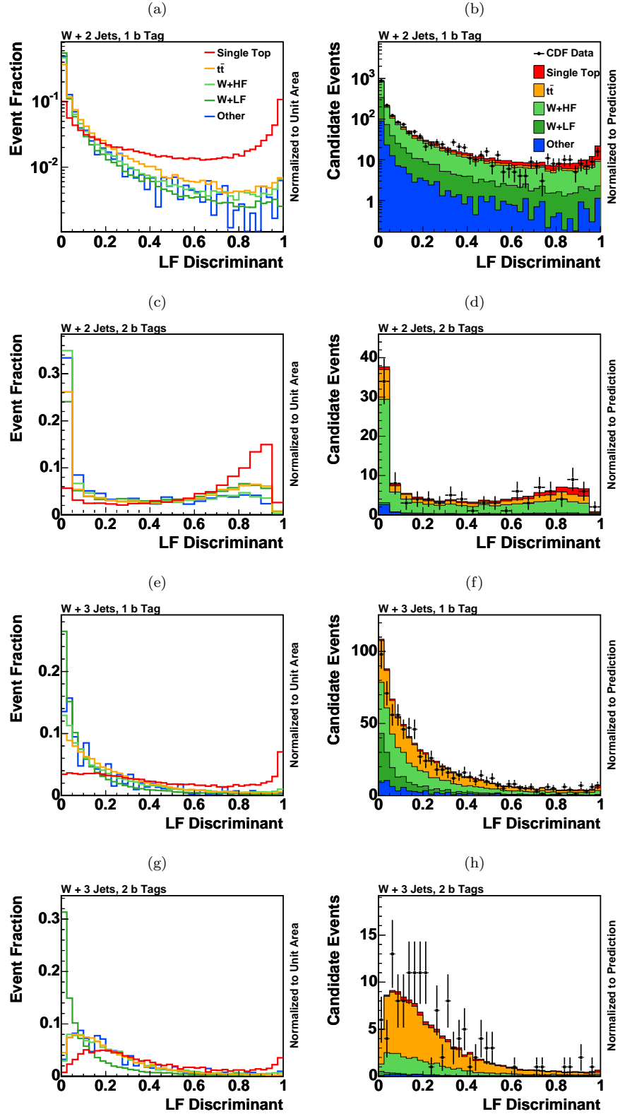
FIG. 21: Templates of predictions for the signal and background processes, each scaled to unit area (left) and comparisons of the data with the sum of the predictions (right) of the likelihood function for each selected data sample. Single top quark events are predominantly found on the right-hand sides of the histograms while background events are mostly found on the left-hand sides. The two-jet, one- b -tag plots are shown on a logarithmic vertical scale for clarity, while the others are shown on a linear scale. The data are indicated by points with error bars, and the predictions are shown stacked, with the stacking order following that of the legend.
