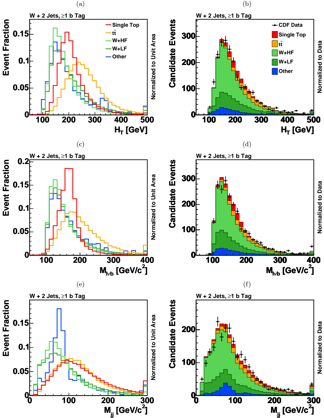
FIG. 19: Monte Carlo templates (left) and validation plots (right) comparing data and Monte Carlo for variables with good discriminating power for events passing our selection requirements with two or three identified jets and at least one b tag. The data are indicated with points, and the shaded histograms show the signal and background predictions which are stacked to form the total prediction. The stacking order follows that of the legend. Overflows are collected in the highest bin of each histogram.
