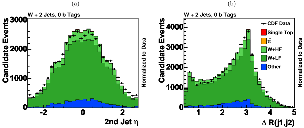
FIG. 34: Graphs showing the poor modeling of the second jet pseudorapidity and the distance between the two jets in the \eta - \phi plane. These are accounted for with systematic uncertainties on the shapes of the W +jets predictions. The data are indicated by points with error bars, and the predictions are shown stacked, with the stacking order following that of the legend.
