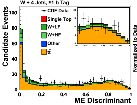
FIG. 26: The event probability discriminant for two-jet one- b -tag events applied to the b -tagged W +four jets control sample, showing that the Monte Carlo t\bar{t} samples model the EPD distribution of the data well. The data are indicated by points with error bars, and the predictions are shown stacked, with the stacking order following that of the legend.
