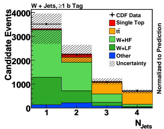
FIG. 15: The number of events predicted and observed for W +jets events in which at least one jet is b -tagged. The data are indicated with points, and the shaded histograms show the signal and background predictions which are stacked to form the total prediction. The stacking order is the same as the legend. The systematic uncertainty on the rates is far too large to use a simple counting experiment to measure the single top quark cross section.
