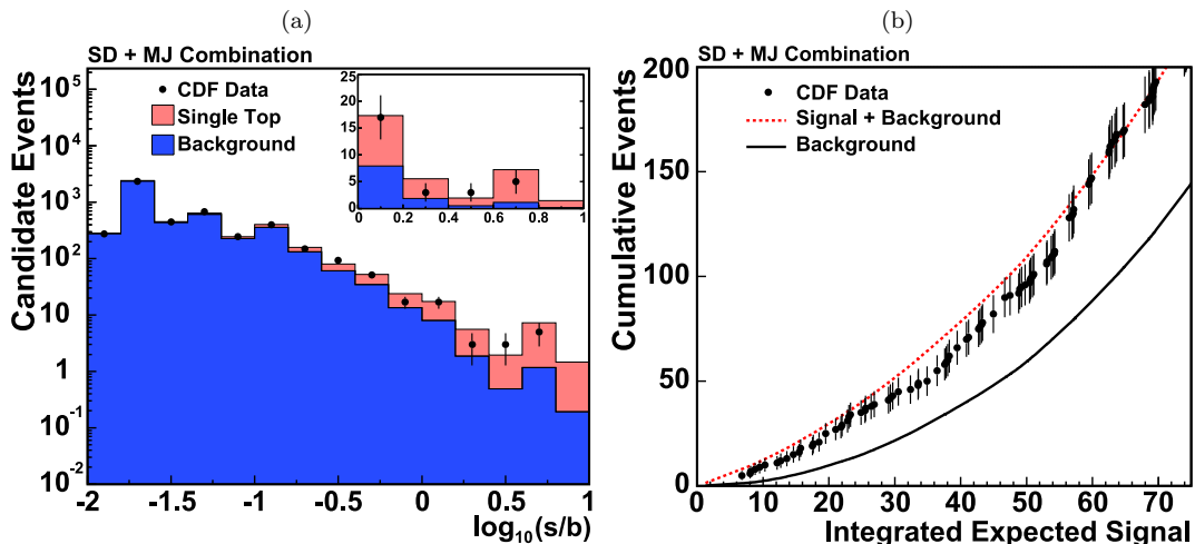
FIG. 38: Distributions of data and predictions for the SD and MJ analyses, where bins of similar s/b have been collected together (left). The points with error bars indicate the observed data, while the stacked, shaded histograms show the predictions, including a standard model single top signal. These distributions are integrated starting on the high- s/b side, and the resulting cumulative event counts are shown on the right, separately for the observed data, for the background-only prediction, and the signal-plus-background prediction.
