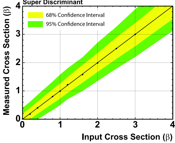
FIG. 35: Check of the bias of the cross-section measurement method using pseudoexperiments, for the super discriminant combination described in Section X. The points indicate the median fit cross section, and the bands show the 68% and 95% quantiles of the distribution of the fitted cross section, as functions of the input cross section. A line is drawn showing equal input and fitted cross sections; it is not a fit to the points.
