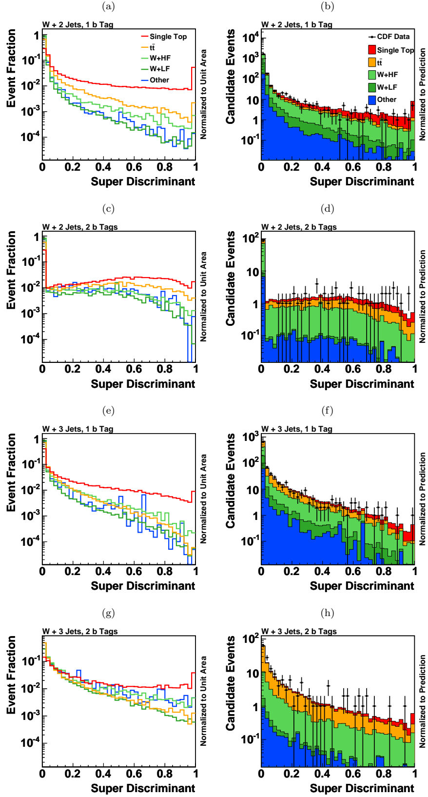
FIG. 36: Normalized templates (left) and plots comparing the predicted distributions with data (right) of the final combined neural network output for each selected data sample. These distributions are more sensitive than any single analysis. The data are indicated by points with error bars, and the predictions are shown stacked, with the stacking order following that of the legend.
