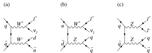
FIG. 10: Feynman diagrams for diboson production, which provides a small background for single top quark production.
