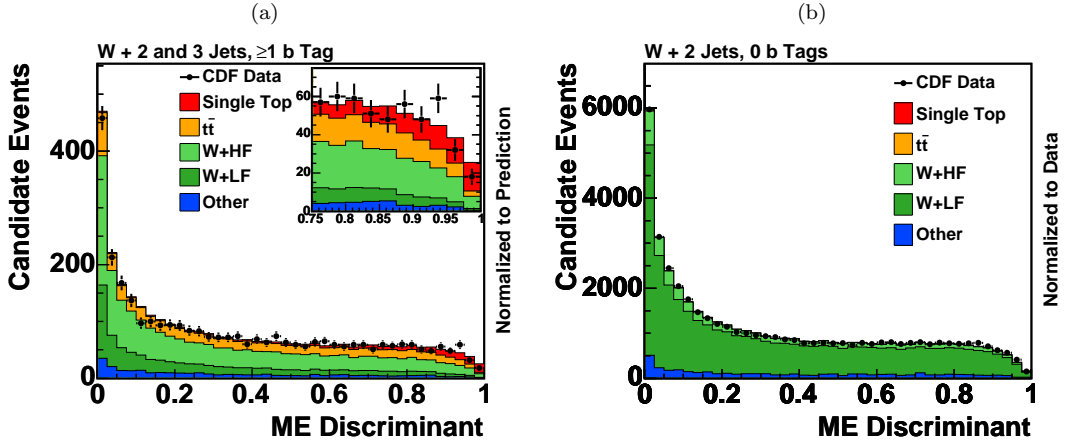
FIG. 25: Comparison of the data with the sum of the predictions of the matrix element discriminant for the sum of all selected data samples (left). The discriminant output for two-jet one- b -tag events applied to the untagged W +two jets control sample (right) shows that the Monte Carlo W +two jets samples model the ME distribution of the data well. The data are indicated by points with error bars, and the predictions are shown stacked, with the stacking order following that of the legend.
