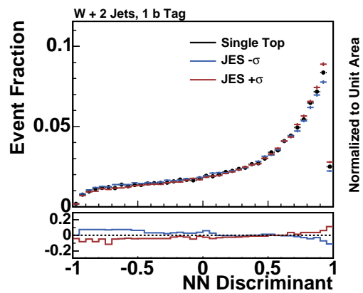
FIG. 33: An example of systematically shifted shape templates. This figure shows the jet energy scale shifted histograms for the single top quark signal in two-jet one- b -tag events for the NN discriminant. The plot below shows the relative difference between the central shape and the two alternate shapes.
