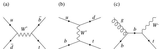
FIG. 1: Representative Feynman diagrams of single top quark production. Figures (a) and (b) are s - and t -channel processes, respectively, while figure (c) is associated Wt production, which contributes a small amount to the expected cross section at the Tevatron.
