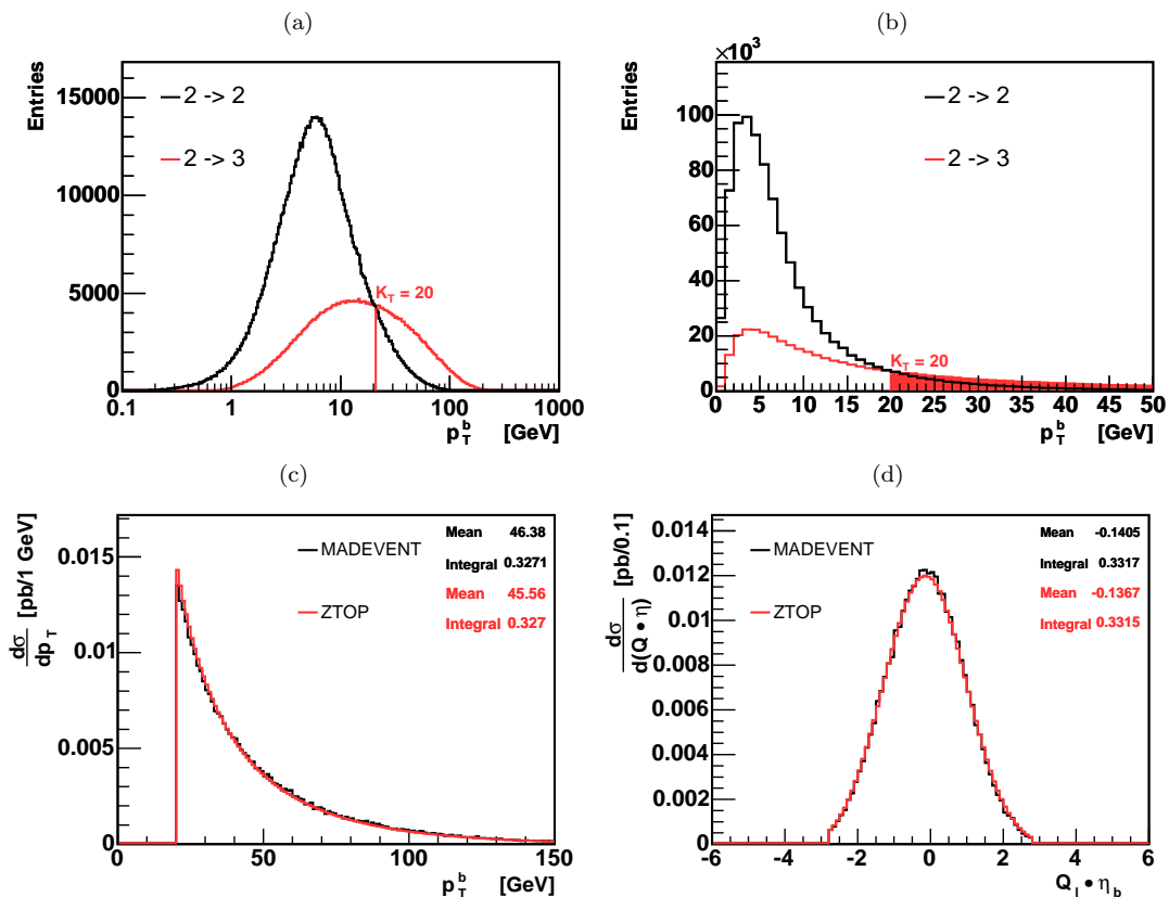
FIG. 7: Matching of t -channel single top quark events of the 2 \rightarrow 2 and the 2 \rightarrow 3 process. The p_T distributions of the spectator b quark are shown, (a) on a logarithmic p_T scale, and (b) on a linear p_T scale. The ratio of 2 \rightarrow 2 to 2 \rightarrow 3 events is adjusted such that the rate of spectator b quarks with p_T > 20 GeV/c and |\eta| < 2.8 matches the theoretical prediction. The fraction of these events is illustrated in (b) by the shaded area. The matched MADEVENT sample reproduces both the rate and the shape of the differential ZTOP p_T (c) and Q_\ell \cdot \eta (d) cross section distributions of the spectator b quark.
