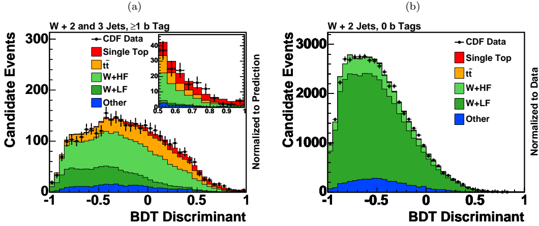
FIG. 31: Comparison of the data with the sum of the predictions of the BDT output for the sum of all selected data samples (left) and the BDT output for two-jet one- b -tag events applied to the untagged two-jet control sample (right), where the dominant contributing process is W +light-flavored jets. The data are indicated by points with error bars, and the predictions are shown stacked, with the stacking order following that of the legend.
