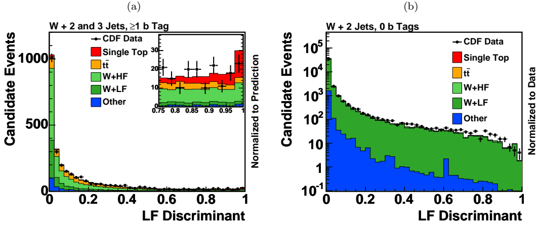
FIG. 22: Comparison of the data with the sum of the predictions of the likelihood function for the sum of all selected data samples (left) and for two-jet one-tag events (right) applied to the untagged sideband, the latter with appropriate modifications to variables that rely on b -tagging. The stacking order follows that of the legend. The discrepancies between the prediction and the observation in the untagged sideband seen here are covered by systematic uncertainties on the W +jets background model.
