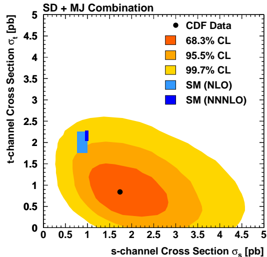
FIG. 40: The results of the two-dimensional fit for \sigma_s and \sigma_t . The black point shows the best fit value, and the 68.3%, 95.5%, and 99.7% credibility regions are shown as shaded areas. The SM predictions are also indicated with their theoretical uncertainties. The SM predictions shown are those of [9, 10] (NLO) and [11] (NNNLO).
