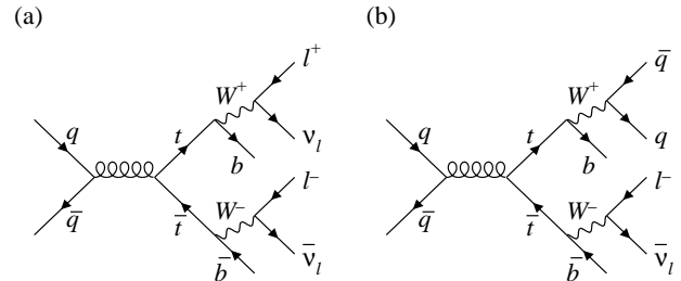
FIG. 9: Feynman diagrams of the t\bar{t} background to single top quark production. To pass the event selection, these events must have one charged lepton (a), or one or two hadronic jets (b), that go undetected.
