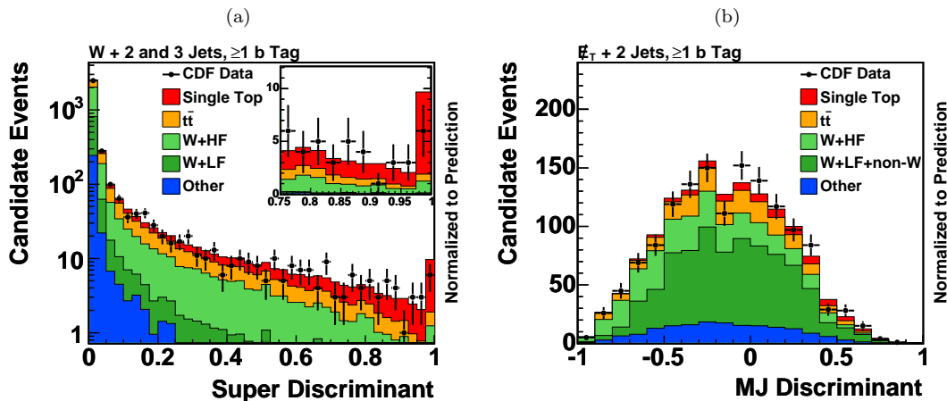
FIG. 37: Comparison of the predicted distributions with data summed over all selected data samples of the super discriminant (left) and the MJ discriminant (right). Points with error bars indicate the observed data, while the stacked, shaded histograms show the predictions, including a standard model single top signal. In each panel, the order of the stacked components follows that of the legend.
