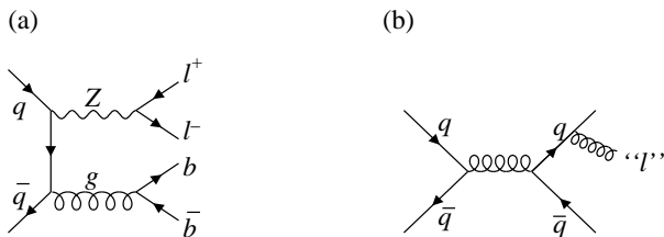
FIG. 11: Representative Feynman diagrams for (a) Z/\gamma^* +jets production and (b) non- W events, in which a jet has to be misidentified as a lepton and \cancel{E}_T must be mismeasured to pass the event selection.
