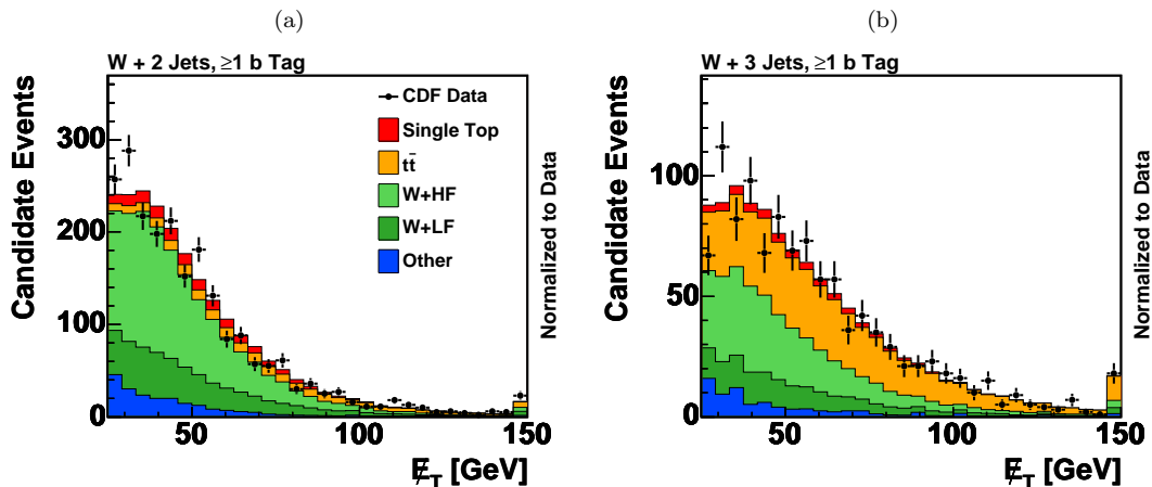
FIG. 18: Validation plots comparing data and Monte Carlo for missing transverse energy for events passing our event selection requirements with two jets (a) and three jets (b), both with at least one b tag. The data are indicated with points, and the shaded histograms show the signal and background predictions which are stacked to form the total prediction. The stacking order follows that of the legend.
