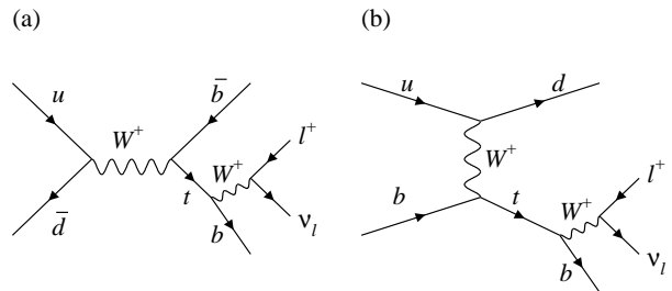
FIG. 3: Feynman diagrams showing the final states of the dominant s -channel (a) and t -channel (b) processes, with leptonic W boson decays. Both final states contain a charged lepton, a neutrino, and two jets, at least one of which originates from a b quark.
