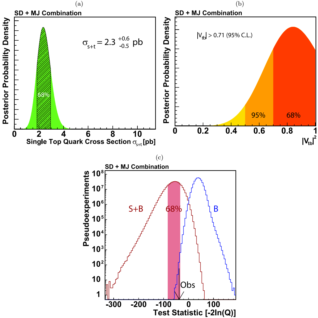
FIG. 39: The posterior curve of the cross section measurement calculated with the super discriminant histograms as inputs (a), the posterior curve for the |V_{tb}| calculation (b), and the distributions of -2 \ln Q in simulated S+B and B -only pseudoexperiments, assuming a Standard Model single top quark signal (c). The value of -2 \ln Q observed in the data is indicated with an arrow.
