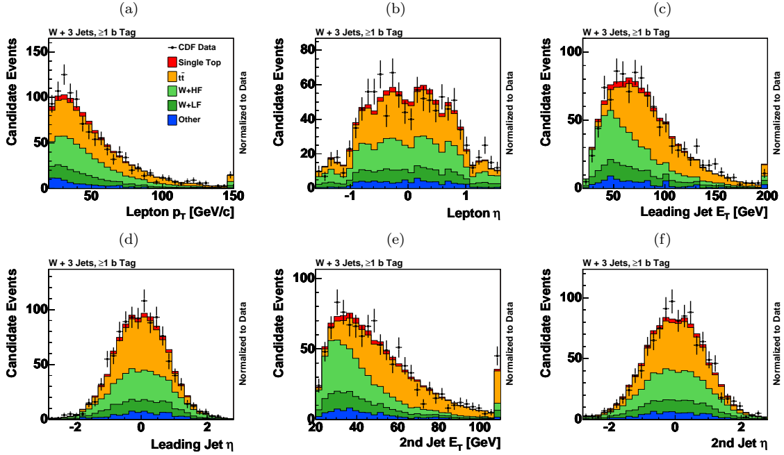
FIG. 17: Validation plots comparing data and Monte Carlo for basic kinematic quantities for events passing the event selection requirements with three identified jets and at least one b tag. The data are indicated with points, and the shaded histograms show the signal and background predictions which are stacked to form the total prediction. The stacking order follows that of the legend.
