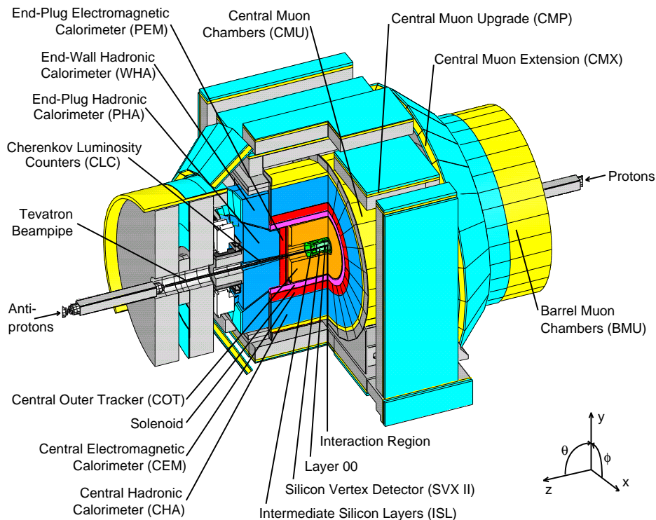
FIG. 2: Cutaway isometric view of the CDF II detector.
