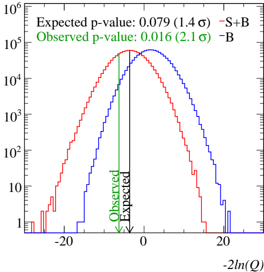
FIG. 12: Distribution of -2 \ln Q for the B or S+B hypothesis. The dark vertical arrow shows the mode of the -2 \ln Q distribution in the S+B hypothesis using pseudoexperiments, while the bright vertical arrow shows the outcome in data. The expected (observed) p -value is the integral of the -2 \ln Q distribution in the B hypothesis at the left of the dark (bright) arrow.
