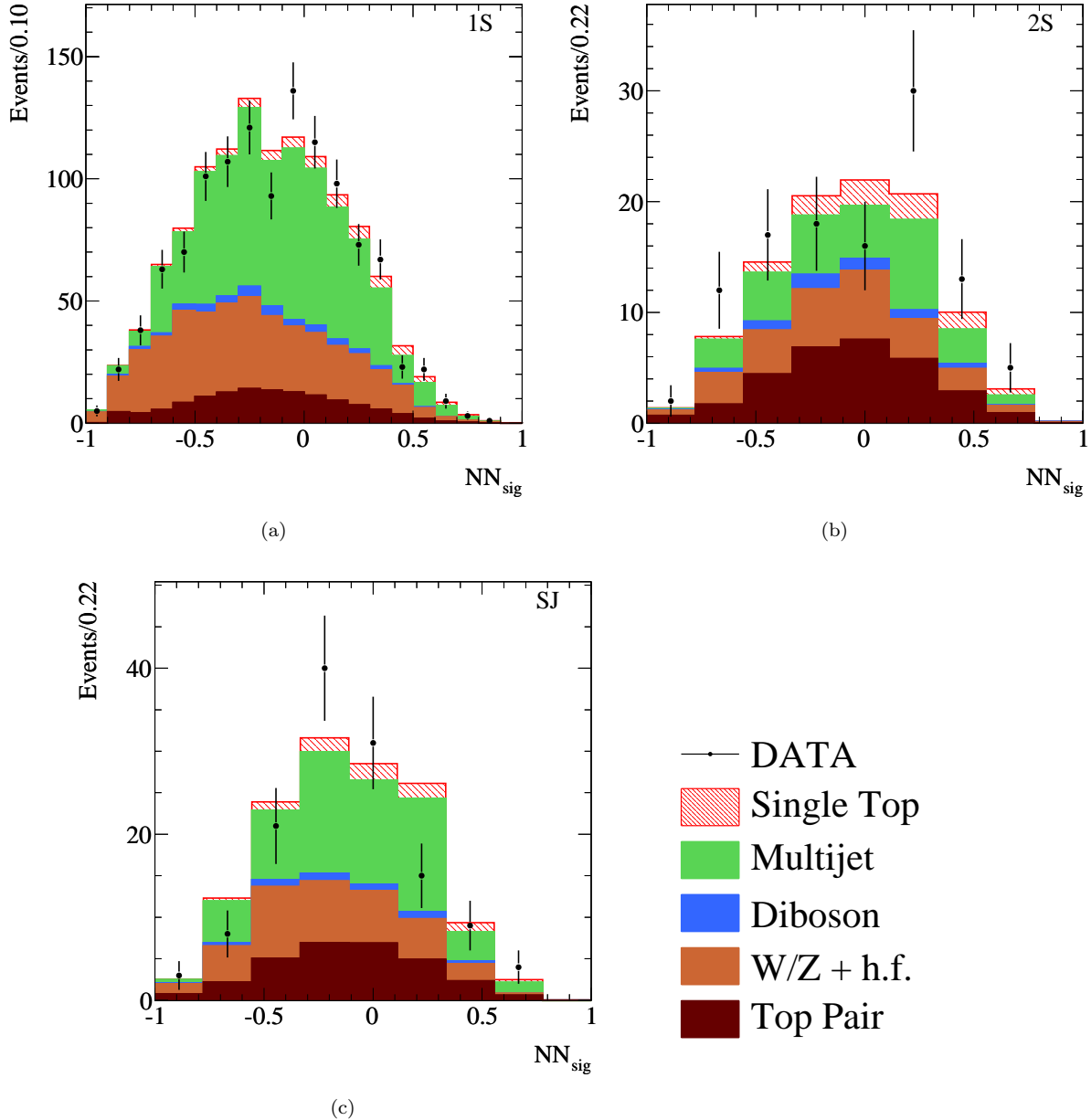
FIG. 10: NN_{\text{sig}} discriminant output distributions in signal region, for the 1S subsample (a), 2S (b), SJ (c).
