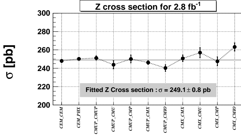
FIG. 3: Z peak cross section measured for each inclusive same flavor dilepton category using the full 2.8 \text{ fb}^{-1} data sample after applying the loose muon scale factor. Not included is a 6% uncertainty in the luminosity measurement common to all channels. The band represents the mean value of 249.1 \pm 0.8 \text{ pb} .
