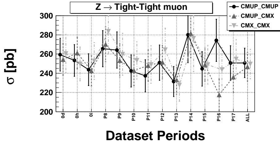
FIG. 2: Z cross section using dilepton categories with tight muons as a function of data taking period.
