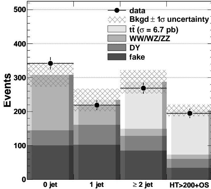
FIG. 9: Dilepton candidate events (black point) by jet multiplicity. The stacked histogram represents the background contribution and the t\bar{t} contribution for an assumed \sigma_{t\bar{t}} = 6.7 \text{ pb} . The hatched area is the uncertainty in the total background estimate.
