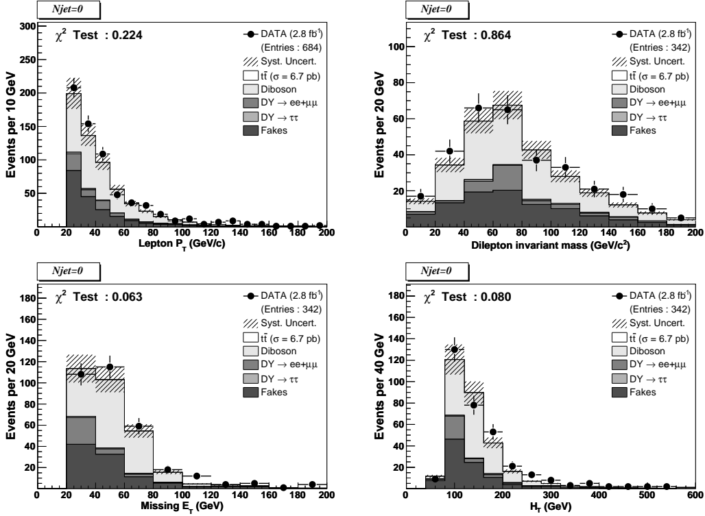
FIG. 5: Background and top quark signal predictions overlaid on the data for 0-jet events in 2.8 \text{ fb}^{-1} . From top left to bottom right: Two leptons transverse energy spectrum, the dilepton invariant mass, the event E_T and H_T . The hatched area represents the uncertainty in the total background estimate.
