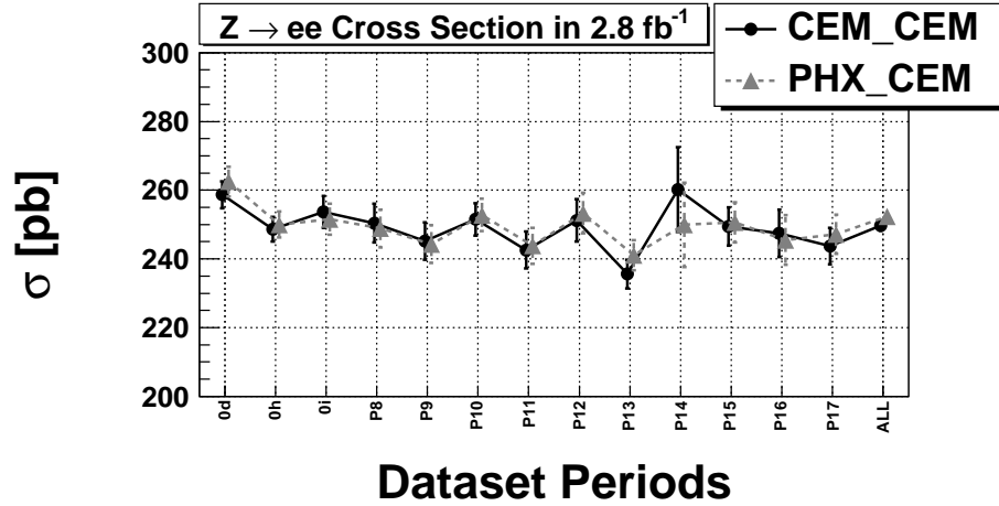
FIG. 1: Z cross section using dilepton categories with two electrons as a function of data taking period.
