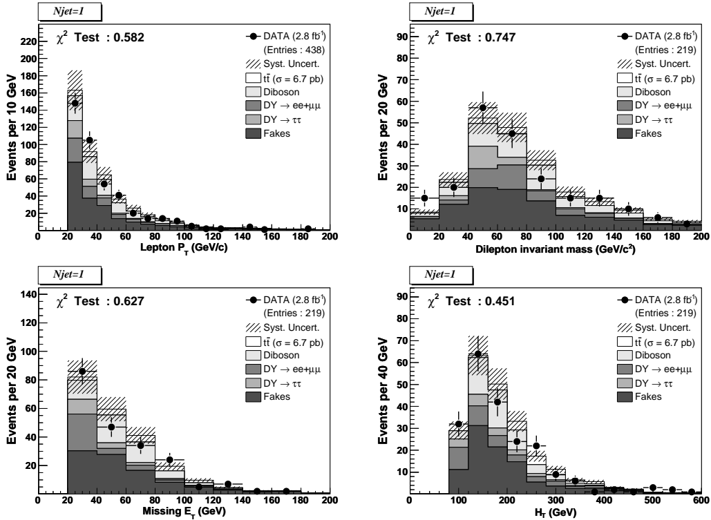
FIG. 6: Background and top quark signal predictions overlaid on the data for 1-jet events in 2.8 \text{ fb}^{-1} . From top left to bottom right: Two leptons transverse energy spectrum, the dilepton invariant mass, the event E_T and H_T . The hatched area represents the uncertainty in the total background estimate.
