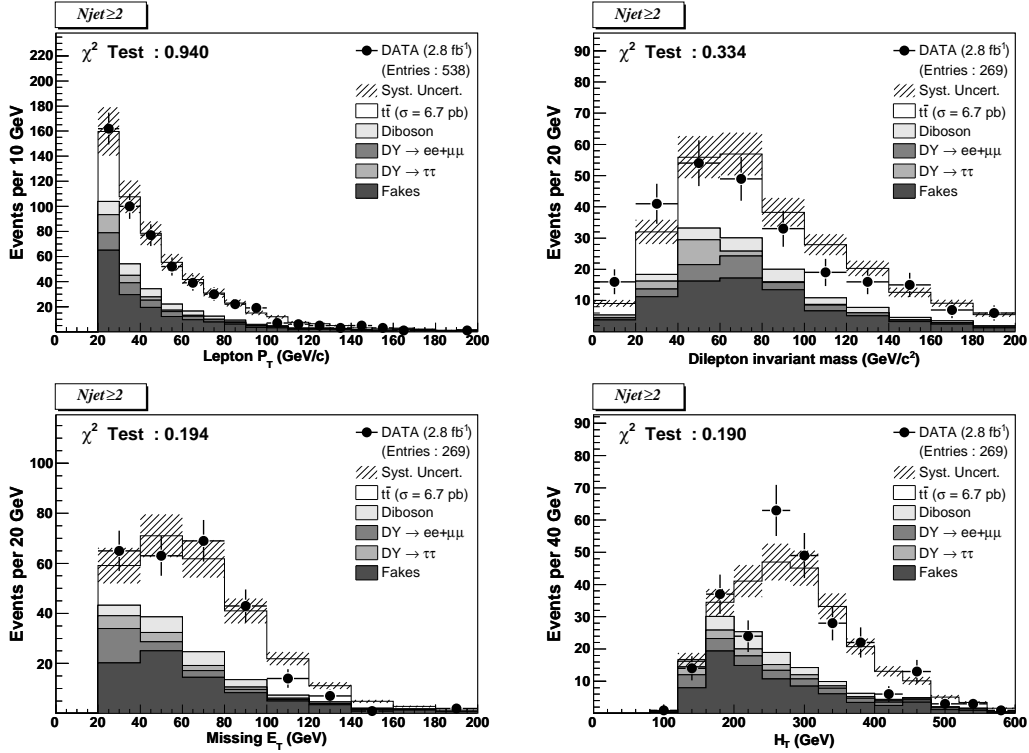
FIG. 7: Background and top quark signal predictions overlaid on the data for 2-jet events before the H_T and the opposite lepton charge requirement in 2.8 \text{ fb}^{-1} . From top left to bottom right: Two leptons transverse energy spectrum, the dilepton invariant mass, the event \cancel{E}_T and H_T . The hatched area represents the uncertainty in the total background estimate.
