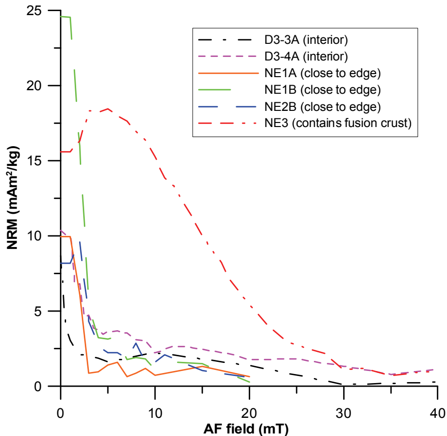
Fig. 7. AF demagnetization curves of NRM of Neuschwanstein interior and edge samples.
