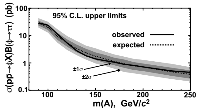
FIG. 2: Observed 95% C.L. upper limits on the cross section for \phi = h/A/H production as a function of m_A . The grey bands show the median expected limit under the null hypothesis, and indicate the \pm 1 - and \pm 2 -standard-deviation ranges.
