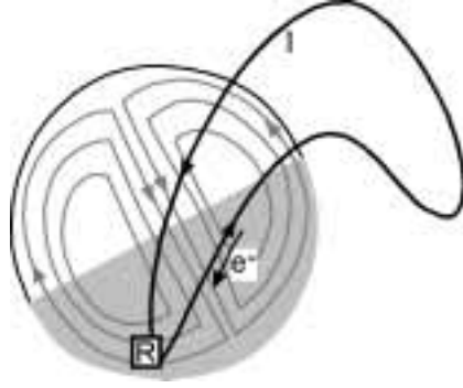
Figure 4.3. A simple current loop, where the field-aligned currents close through the ionospheric load. See text for explanation.
