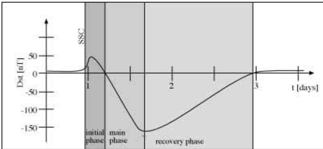
Figure 2.2. Evolution of the Dst index during a magnetic storm.
