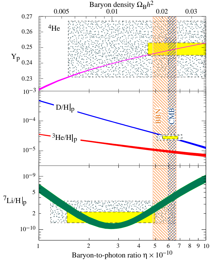
Figure 2.1: The abundances of {}^4\text{He} , \text{D} , {}^3\text{He} and {}^7\text{Li} as predicted by the standard model of big-bang nucleosynthesis — the bands the 95% range. Boxes indicate the observed light element abundances (smaller boxes: \pm 2\sigma statistical errors; larger boxes: \pm 2\sigma statistical and systematic errors). The narrow vertical band indicates the CMB measure of the cosmic baryon density, while the wider band indicates the BBN concordance range (both at 95% CL). Image courtesy of Particle Data Group.
