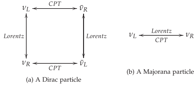
Figure 3.1: The difference between Dirac and Majorana fermions in a nutshell.
