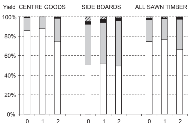
Figure 13. The simulated sawn timber yield (centre goods, side boards and total volume) by quality grades for different thinning treatments (0 unthinned, 1 normal and 2 intensive thinning). Stack colours for quality grades: A (white), B (grey), C (black) and D (striped) (Study V).
