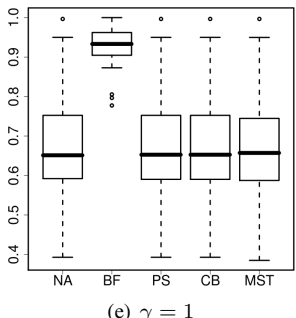
Figure 3. Ratio of connectivity kept by each of the four algorithmic variants. Each boxplot shows the distribution of results over 30 test graphs. NA = Naive approach, BF = Brute Force, PS = Path Simplification, CB = Combinational approach, MST = Maximum Spanning Tree.
