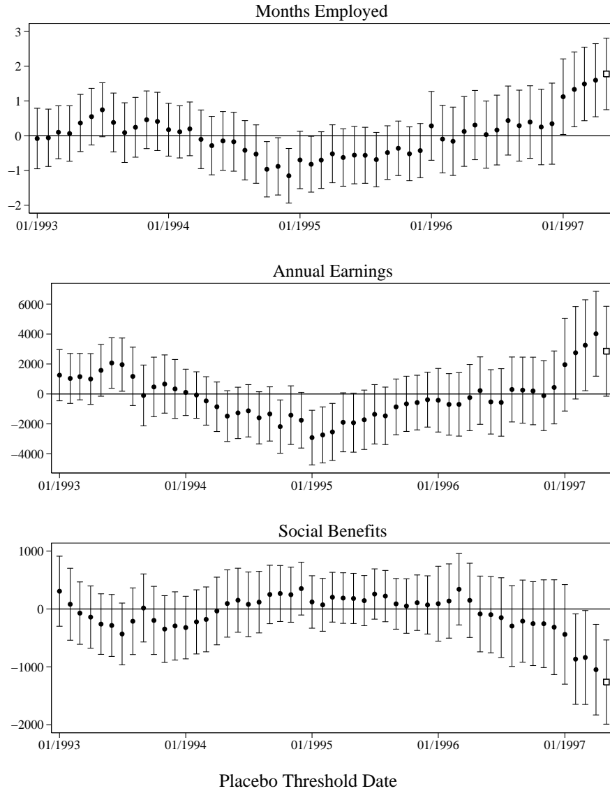
Figure 4: Jumps at non-discontinuity points
