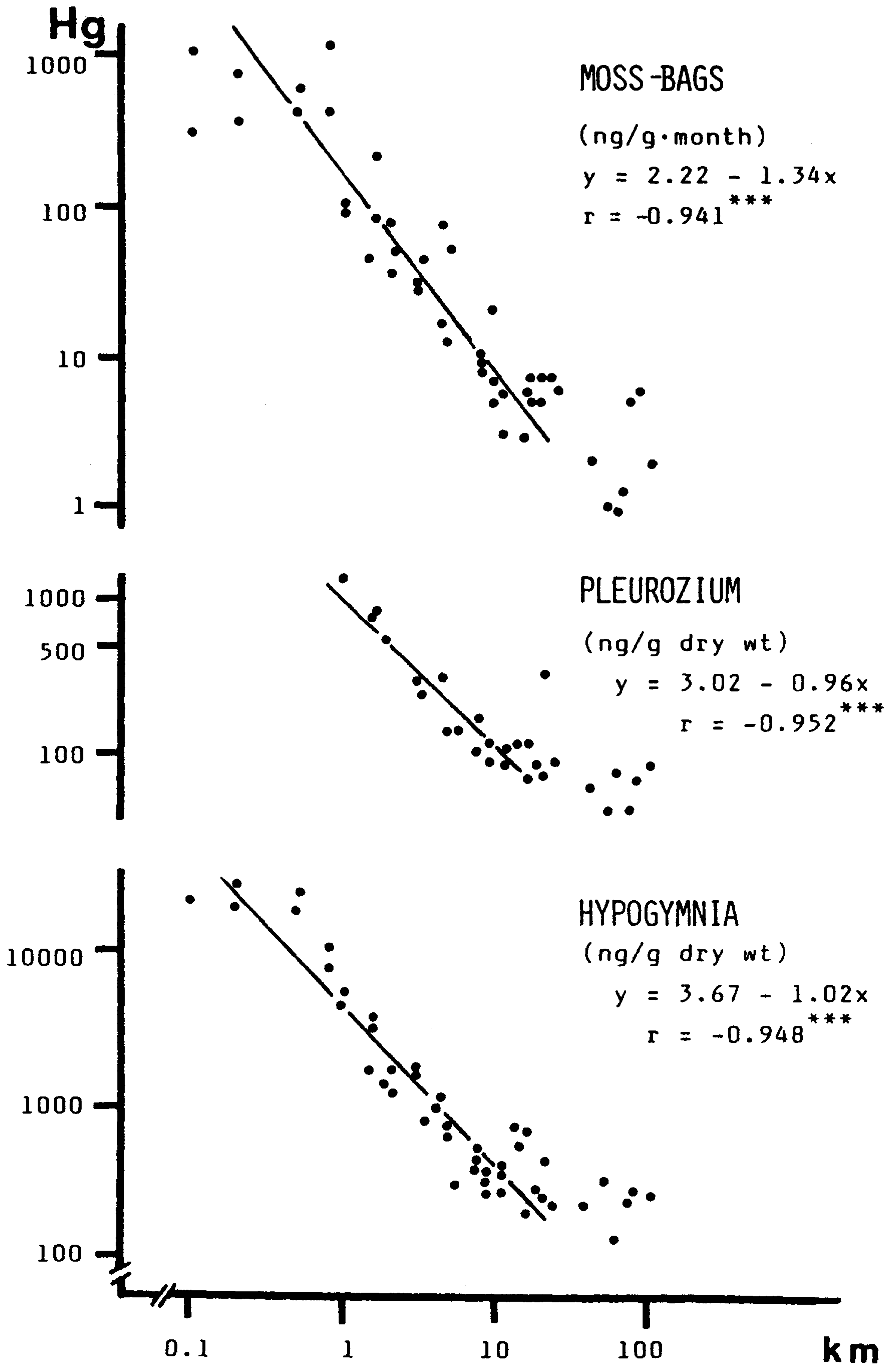
Fig. 2. The mercury accumulation in moss-bags and the mercury contents of Pleurozium schreberi and Hypogymnia physodes at different distances from the chlor-alkali plant. The correlations are calculated from data 0-20 km.
