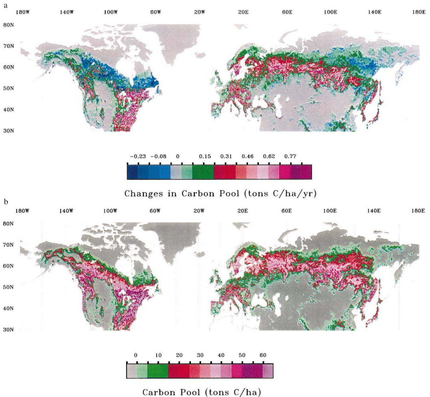
Fig. 2. Spatial detail of changes in the woody biomass carbon pool of northern temperate and boreal forests between late 1990s and early 1980s ( a ) and pool size during late 1990s ( b ). Biomass estimates were converted to carbon by multiplying by 0.5, a standard factor for converting woody biomass to carbon (4, 5).
