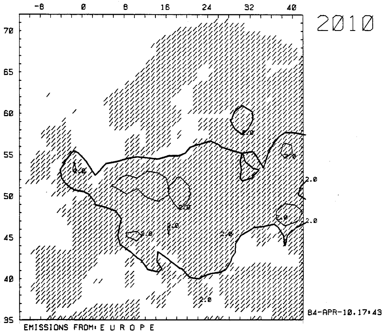
Figure 4-13. Comparison of computed sulfur deposition in example 3.
