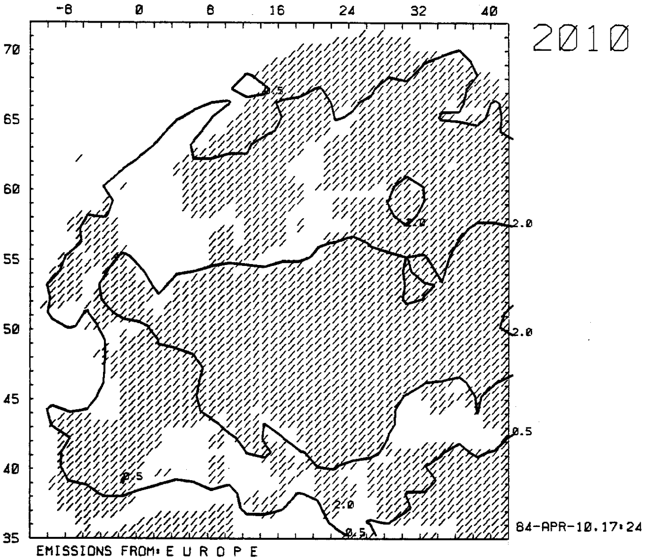
Figure 4-5. Total sulfur deposition in the year 2010 computed in example 1. The isolines of 0.5 and 2.0g · m -2 · yr -1 are shown.
