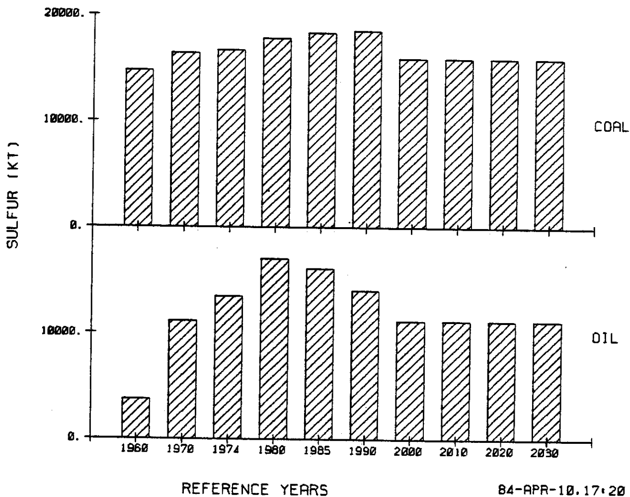
Figure 4-4. Graphical summary of computed sulfur emissions .
