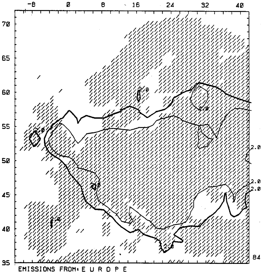
Figure 4-10. Comparison of computed sulfur deposition in example 2. The isoline of 2.0 \text{ g} \cdot \text{m}^{-2} \cdot \text{yr}^{-1} is shown.
