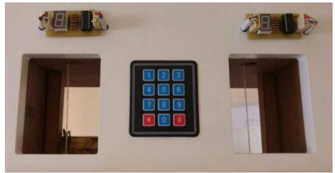
Fig. 9 The cabins, display and numerical keypad
