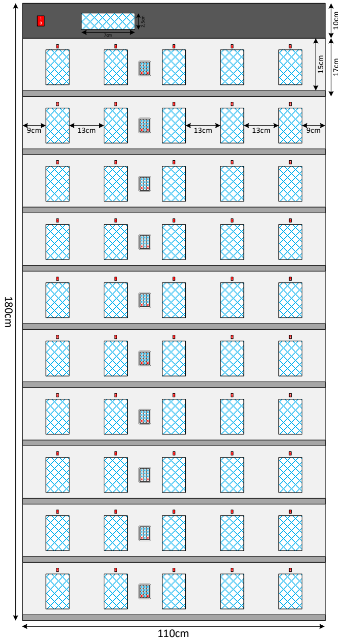
Fig. 5 Designed group elevator system
