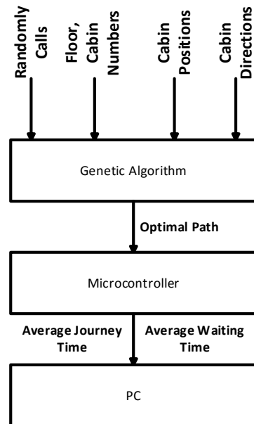
Fig. 6 The flowchart of proposed approach
