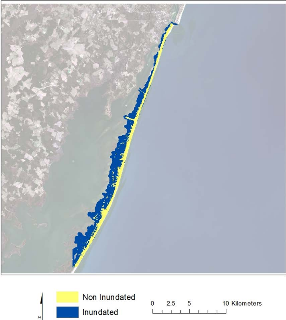
Figure 14. Assateague Island National Seashore inundation levels under IPCC RCP8.5 scenario.
