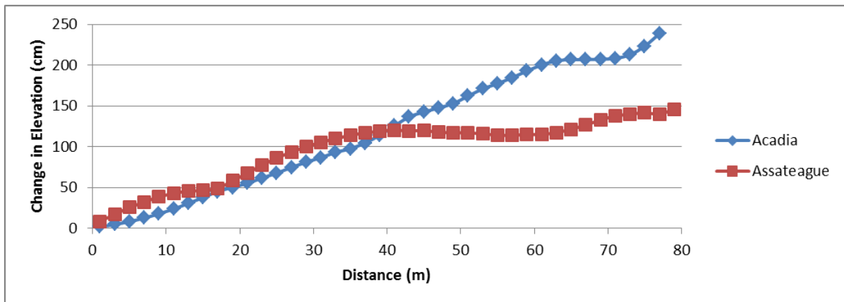
Figure 4. Beach profiles of Sand Beach at Acadia National Park and South Ocean Beach at Assateague Island National Seashore.
