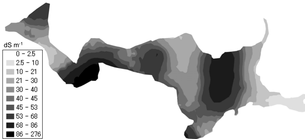
Fig.10. Distribution of the groundwater EC in area 4 in 1977
