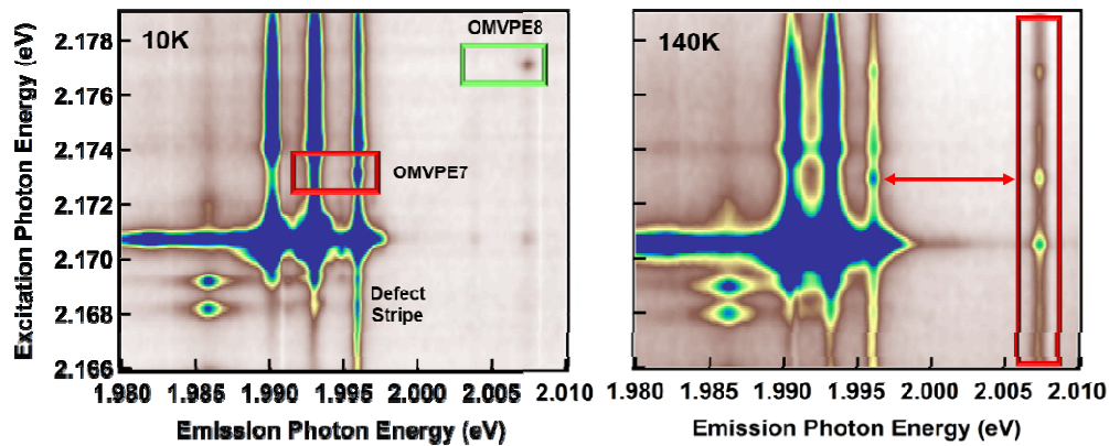
FIG. 3. CEES maps of a GaN:Eu sample grown with a V/III ratio of 3200 at 10K and 140K. At 140K, the emission from the defect stripe is shared between Eu2 and OMVPE8. Also, the emission from Eu2 occurs as the resonant excitation energy of OMVPE8 and vice versa as it did in FIG. 1.
