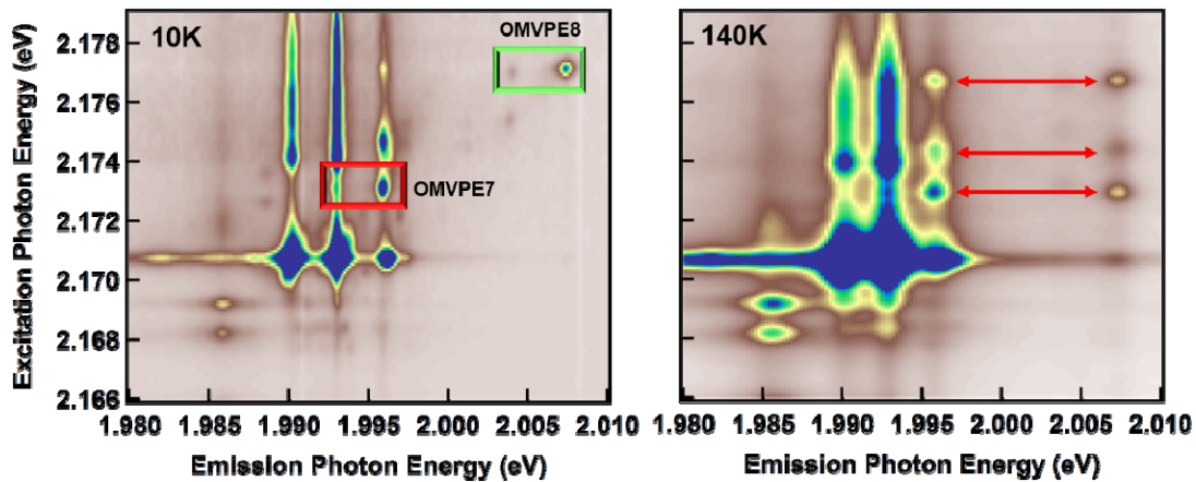
FIG. 2. CEES maps of a GaN:Eu sample grown with a V/III ratio of 6400 at 10K and 140K. At 140K, the emission from Eu_2 occurs as the resonant excitation energy of OMVPE8 and vice versa, suggesting a link between the two centers.
