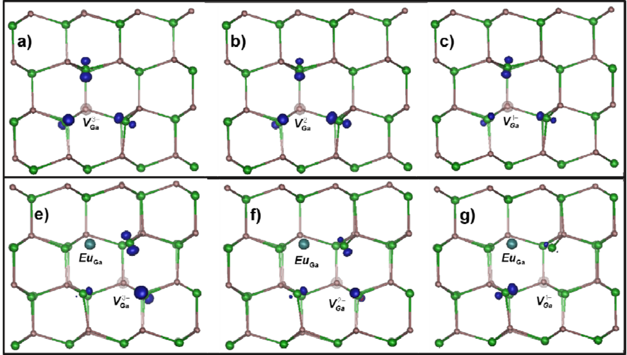
FIG. 1. (a-c) Spatial distribution of the electron charge density around a V_{\text{Ga}} for the case where the vacancy has captured one to three excess electrons, respectively. (e-g) Spatial distribution of the electron charge density around V_{\text{Ga}} - \text{Eu} complexes which have captured one to three excess electrons, respectively. The isosurfaces of charge density are plotted at 0.1e/\text{\AA}^3 for V_{\text{Ga}}^{2-} and V_{\text{Ga}}^{3-} and at 0.06e/\text{\AA}^3 for V_{\text{Ga}}^{-} .
