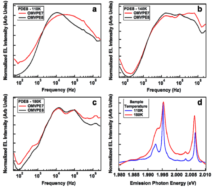
FIG. 5. Frequency response curves for Eu2 and Eu2* acquired from PDES measurements taken at: (a) 110K, (b) 140K, and (c) 180K. The emission spectra at the peak frequency of Eu2*, at 110K and 180K is given in (d).
