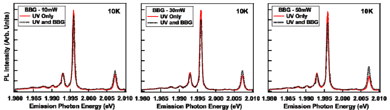
FIG. 6. Comparison of the emission spectra of the GaN:Eu sample with a V/III ratio of 3200 under 325nm (UV) excitation alone and overlapped with 532nm (BBG) excitation. The 532nm laser can excite the \text{Eu}^{3+} ions through the defect-stripe observed in Figure 3. The excitation power of the 532nm laser was increased from 10mW – 50mW at 10K. The conversion of \text{Eu}^{2+} into \text{Eu}^{2*} is clearly observed for a BBG excitation power of 50mW.
