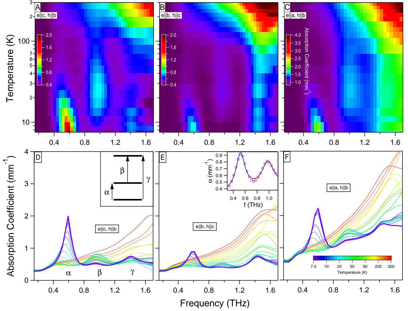
FIG. 1. (Color Online) Spin-Orbital THz absorption of \text{Sr}_2\text{FeSi}_2\text{O}_7 . False color maps of the absorption from 7.5 K to 300 K and below 1.7 THz for the (A) e_\omega \parallel c, h_\omega \parallel b , (B) e_\omega \parallel b, h_\omega \parallel c , and (C) e_\omega \parallel a, h_\omega \parallel b configurations. The color corresponds to the absorption value as indicated in the scale bar in each individual panel. (D)-(F) Selected absorption traces for the same polarization configurations as in (A)-(C), respectively. The color scale bar in (D) applies to the three (D) through (F) panels. Please note that the temperature spacing between each line are not equally separated, but follow a semi-logarithmic increment from the lowest temperature. Inset in (D) shows the three level structure that is apparent in the temperature dependence of the absorption. Transitions are labeled as \alpha , \beta , and \gamma as indicated. A different absorption mode appears at higher T, and dominates the other three. The inset in (E) shows an example of the raw spectrum (red square) at 15 K for e_\omega \parallel c, h_\omega \parallel b along with its fitted line (solid blue).
