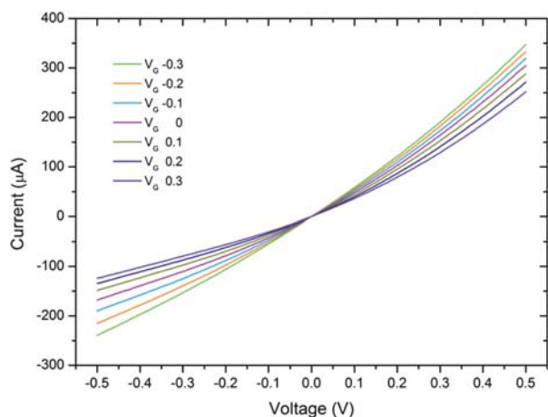
Fig. 3 Electrical characteristics of suspended SWNT-films at various electrolyte gate voltages from -0.3\ \text{V} to 0.3\ \text{V} .
