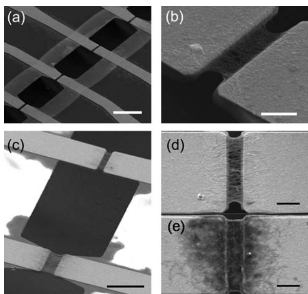
Fig. 2 SEM images of suspended SWNT-film arrays at the magnifications of (a) \times 400 (scale bar: 50\ \mu\text{m} ) and (b) \times 5,000 (scale bar: 5\ \mu\text{m} ). (c) SEM image of suspended SWNT-films with a different channel length (scale bar: 20\ \mu\text{m} ). SEM images of aptamer functionalized SWNT-films (d) before and (e) after thrombin binding (scale bars: 5\ \mu\text{m} ).
