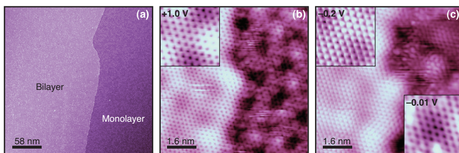
FIG. 5: (a) Large scale STM image taken with +2 V and 50 pA, where two wide domains of monolayer and bilayer graphene are clearly distinguished. (b),(c) STM images at the boundary of monolayer (right) and bilayer domains (left), taken with two different bias voltages marked at the upper left. Insets at the upper left show magnified images of the left domains. The full honeycomb pattern at high-bias voltage (b) transforms into the triangular pattern at low-bias voltage (c), which is the characteristic bias dependence in bilayer graphene reported previously [20]. This confirms the bilayer origin of domains under study. The lower right inset in (c) shows a magnified low-bias (marked) image of the right domains, showing a clear honeycomb lattice of monolayer graphene.
