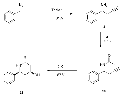
Scheme 3 A protective group-free synthesis of piperidin-4-ol from benzylic azide. a \text{CH}_3\text{COCl} (1.2 equiv.), \text{Et}_3\text{N} (2 equiv.), \text{CH}_2\text{Cl}_2 , rt, 5 h. b [\text{Au}(\text{PPh}_3)]^+\text{NTf}_2^- (5 mol%), \text{MsOH} (1.2 equiv.), 4 Å M.S., rt, 20 min; catecholborane (6 equiv.), rt, 10 h.
