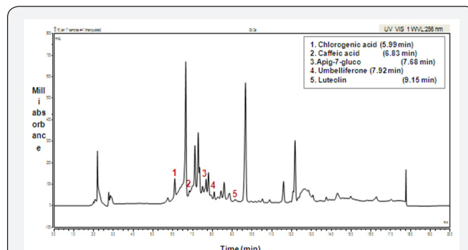
Figure 2: The HPLC-UV chromatogram of phenol and flavonoid compounds content of chamomile leaves detected at 256 nm under drought stress conditions.
