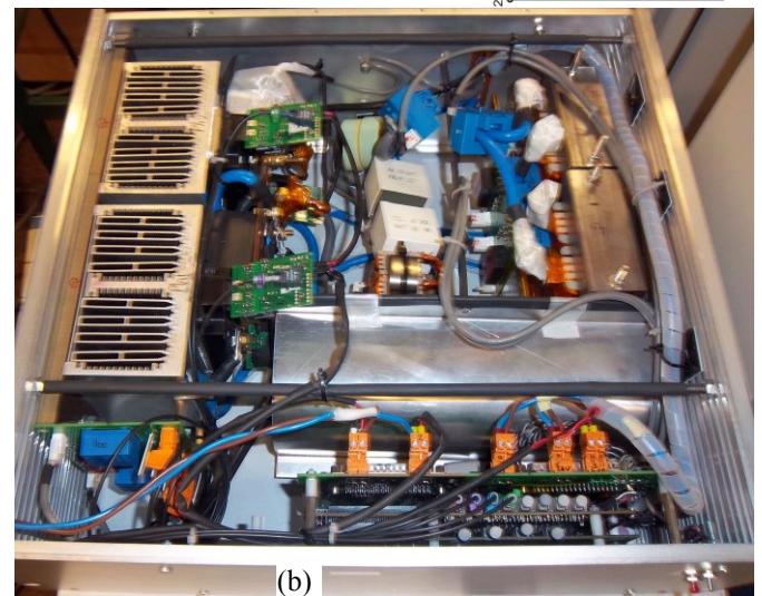
Fig. 8: a) Schematic of the battery energy storage system; b) Actual implementation of the converter (BDCR box).
