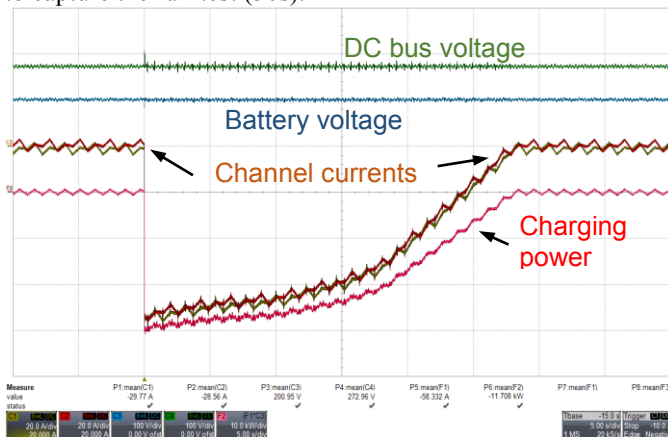
Fig.11: Experimental result of the battery converter processing the specified braking power profile.
