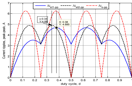
Fig. 7: Peak-peak channel current ripples for the various stages at different duty cycles.
