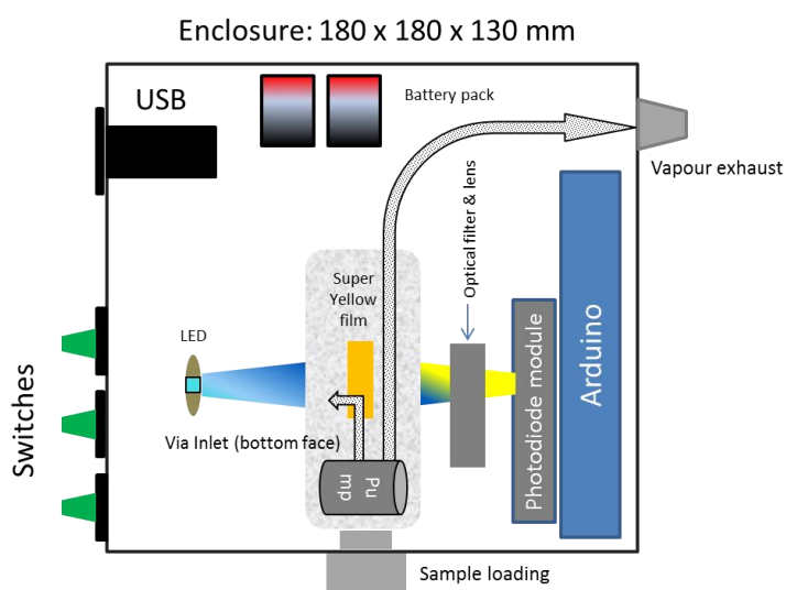
Fig. 2. (a) Schematic of instrumentation (not to scale); (b) Photograph of Enclosure with labelled parts; (c) Loading mechanism with a Merck Super Yellow film.
