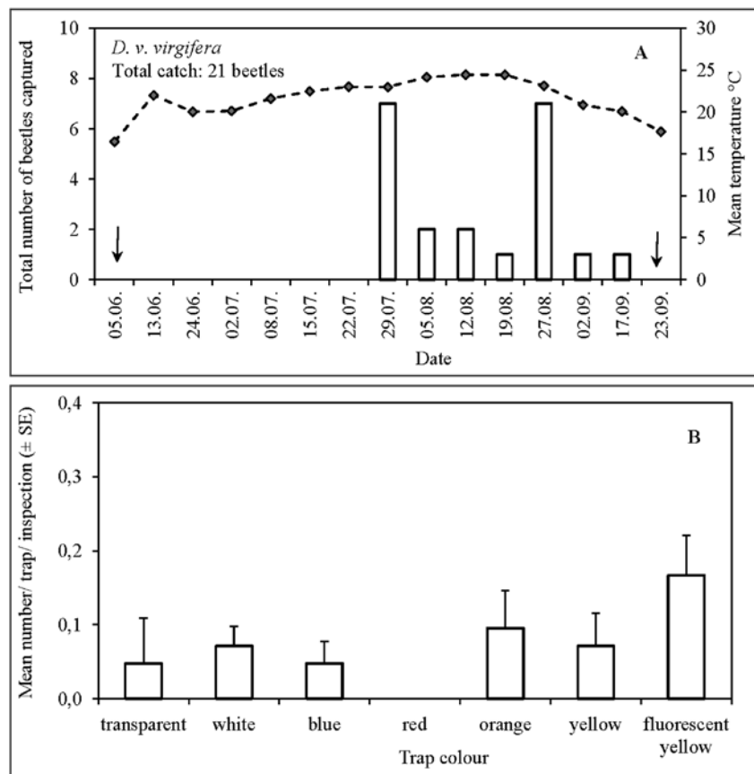
Fig. 3. Seasonal activity of the adults of Diabrotica virgifera virgifera in Knezha in 2014 (A); distribution of the mean captures in transparent and coloured sticky traps (B). For the legend, see Fig. 2
