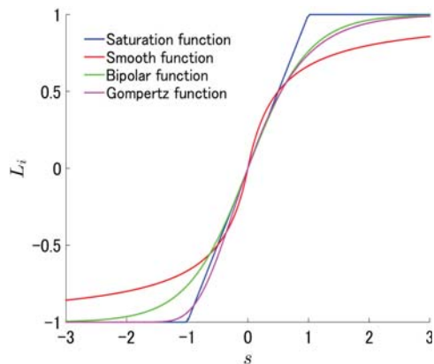
Fig. 3 Candidate functions
