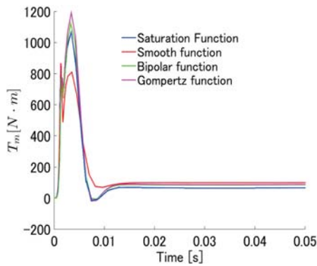
Fig. 6 Enlarged view of time response of driving torque on icy road (( 0 < t < 0.05 ))
