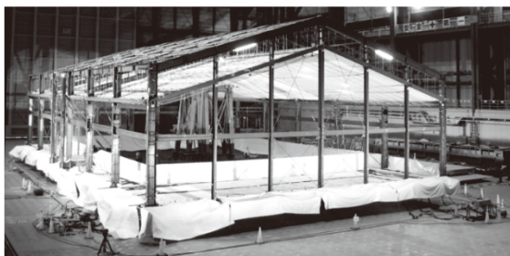
Fig. 4 Gymnasium specimen 8)
